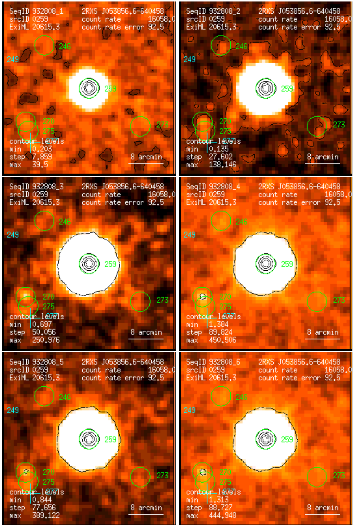
Figure 259: RASS 932808: detection 0259: band rate images, Gaussian filter: (1) PSPC channels 11 – 41, (2) 52 – 90, (3) 91 – 201, (4) 11 – 235, (5) 52 – 201, (6) 11 – 201. Broad band rates in counts/ks. Band rate contour levels in counts/ks/arcmin 2 .
