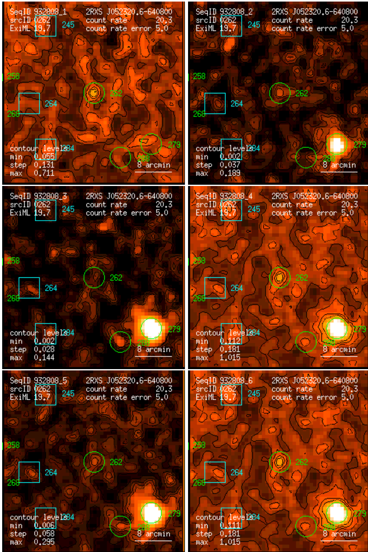
Figure 262: RASS 932808: detection 0262: band rate images, Gaussian filter: (1) PSPC channels 11 – 41, (2) 52 – 90, (3) 91 – 201, (4) 11 – 235, (5) 52 – 201, (6) 11 – 201. Broad band rates in counts/ks. Band rate contour levels in counts/ks/arcmin 2 .
