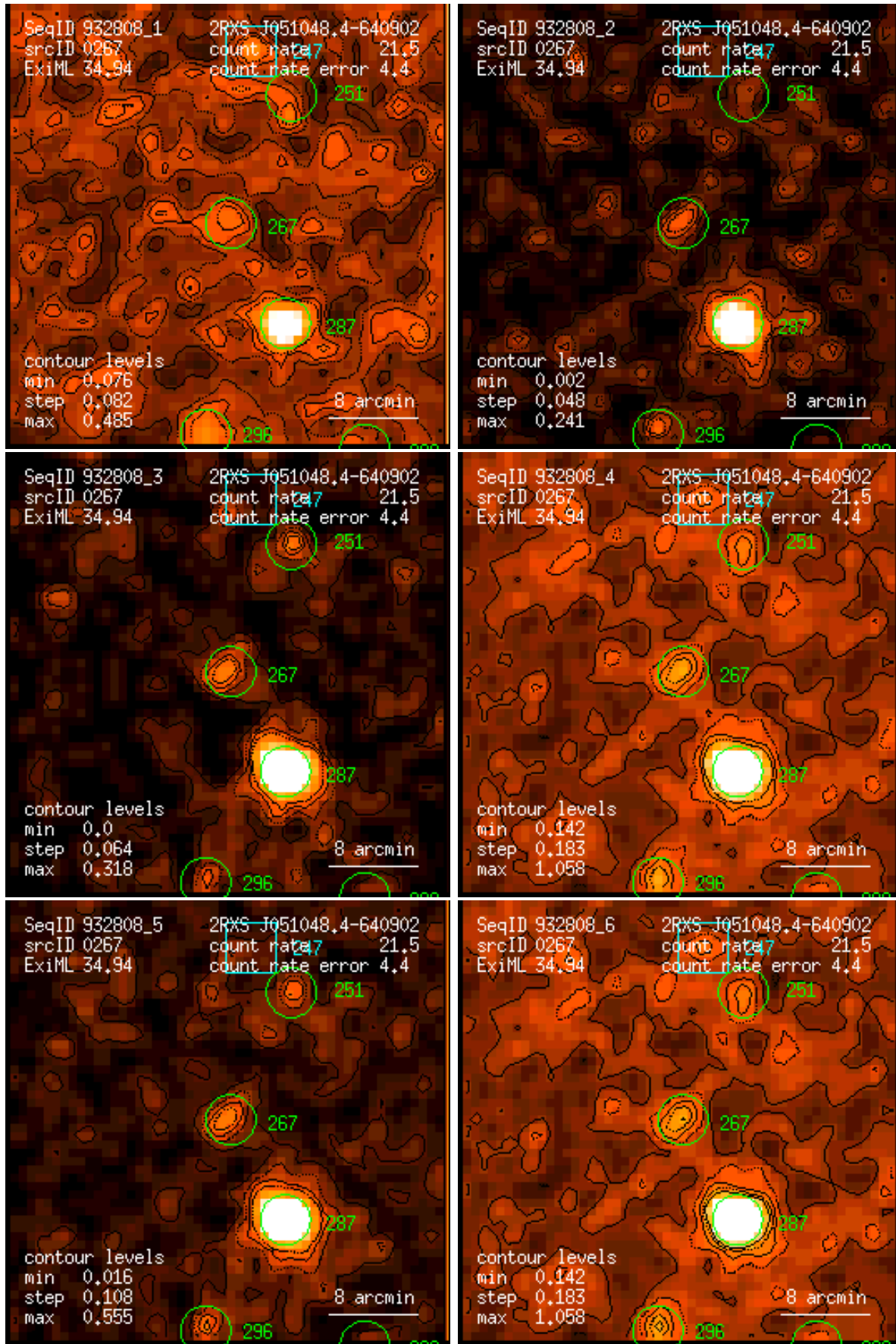
Figure 267: RASS 932808: detection 0267: band rate images, Gaussian filter: (1) PSPC channels 11 – 41, (2) 52 – 90, (3) 91 – 201, (4) 11 – 235, (5) 52 – 201, (6) 11 – 201. Broad band rates in counts/ks. Band rate contour levels in counts/ks/arcmin 2 .
