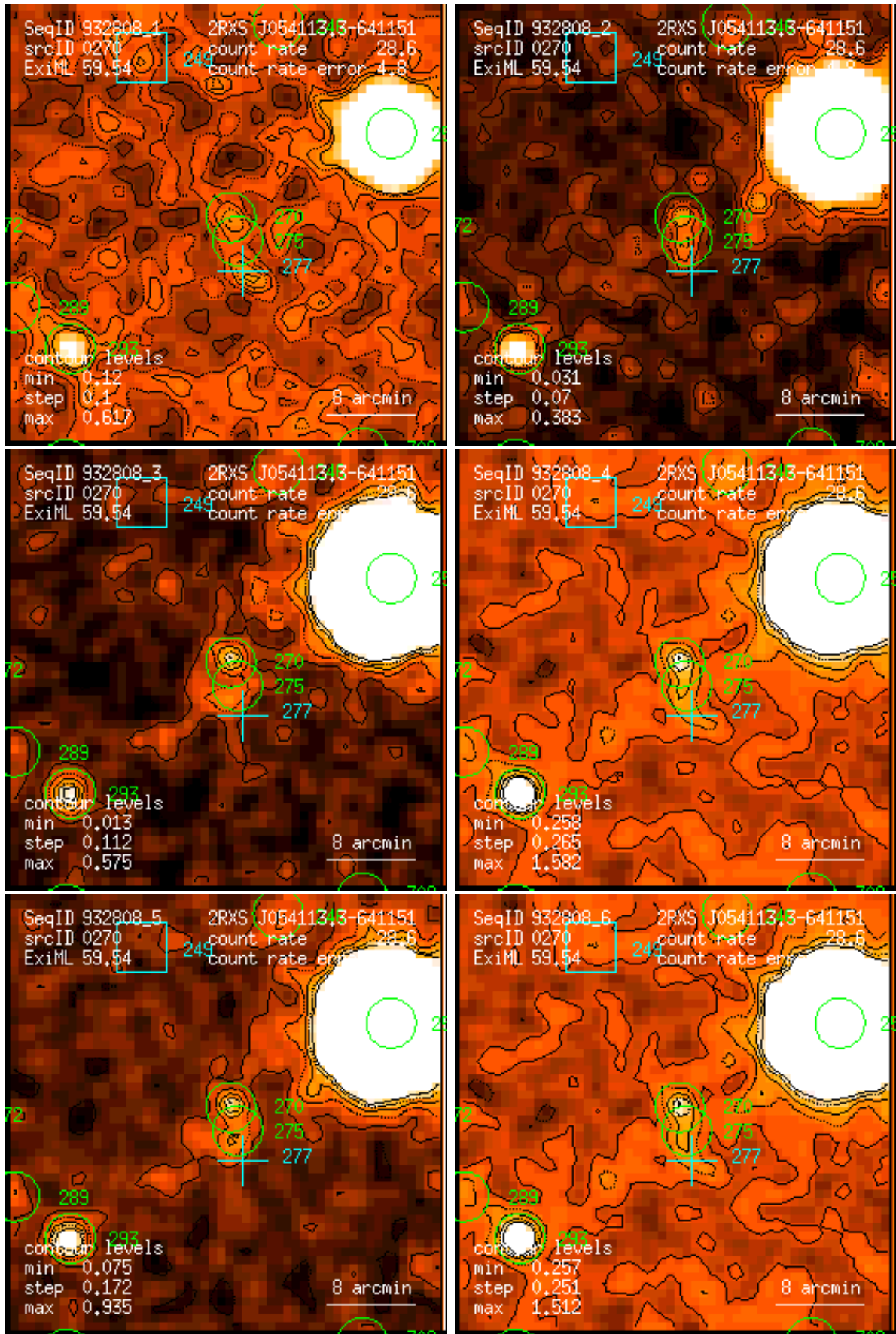
Figure 270: RASS 932808: detection 0270: band rate images, Gaussian filter: (1) PSPC channels 11 – 41, (2) 52 – 90, (3) 91 – 201, (4) 11 – 235, (5) 52 – 201, (6) 11 – 201. Broad band rates in counts/ks. Band rate contour levels in counts/ks/arcmin 2 .
