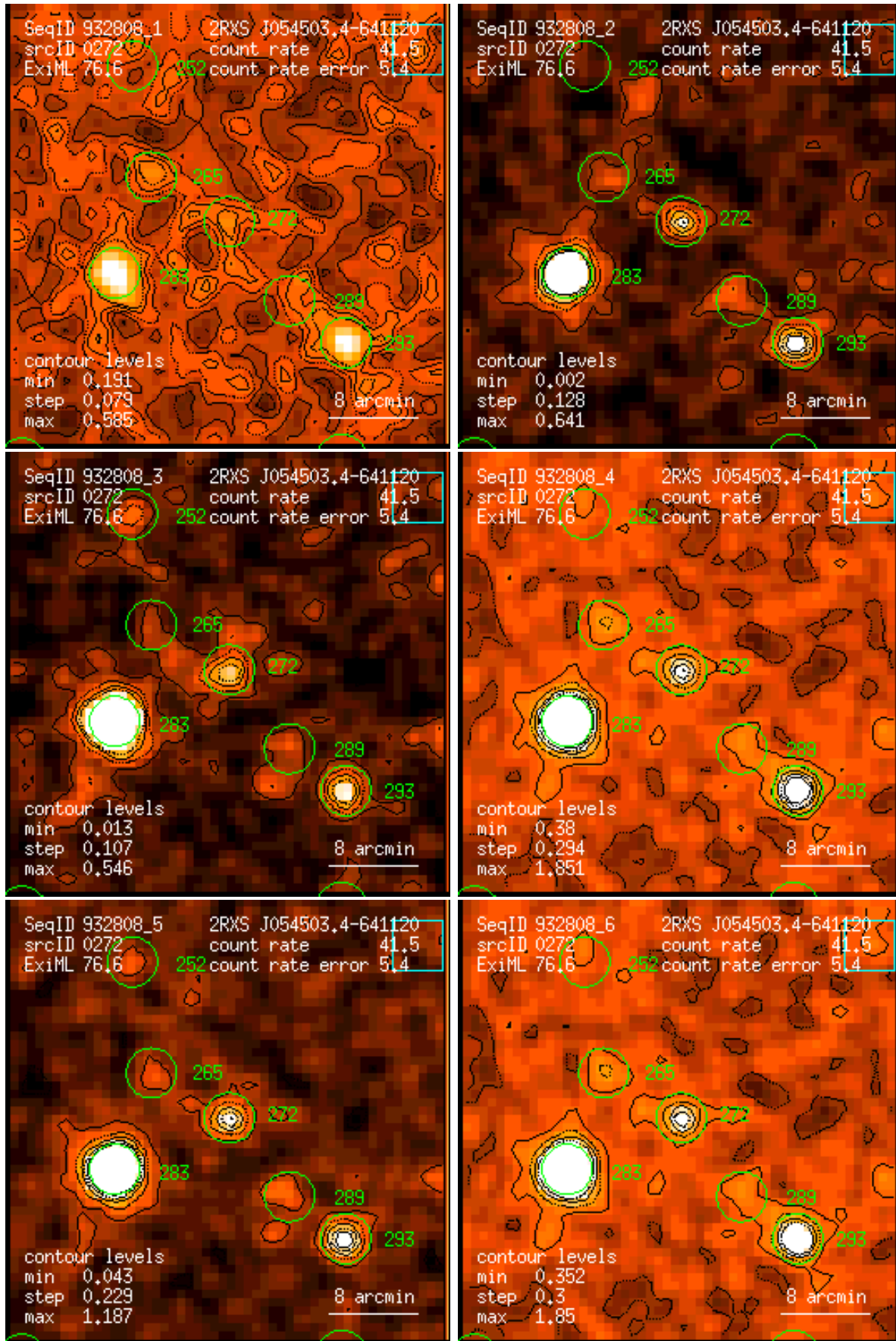
Figure 272: RASS 932808: detection 0272: band rate images, Gaussian filter: (1) PSPC channels 11 – 41, (2) 52 – 90, (3) 91 – 201, (4) 11 – 235, (5) 52 – 201, (6) 11 – 201. Broad band rates in counts/ks. Band rate contour levels in counts/ks/arcmin 2 .
