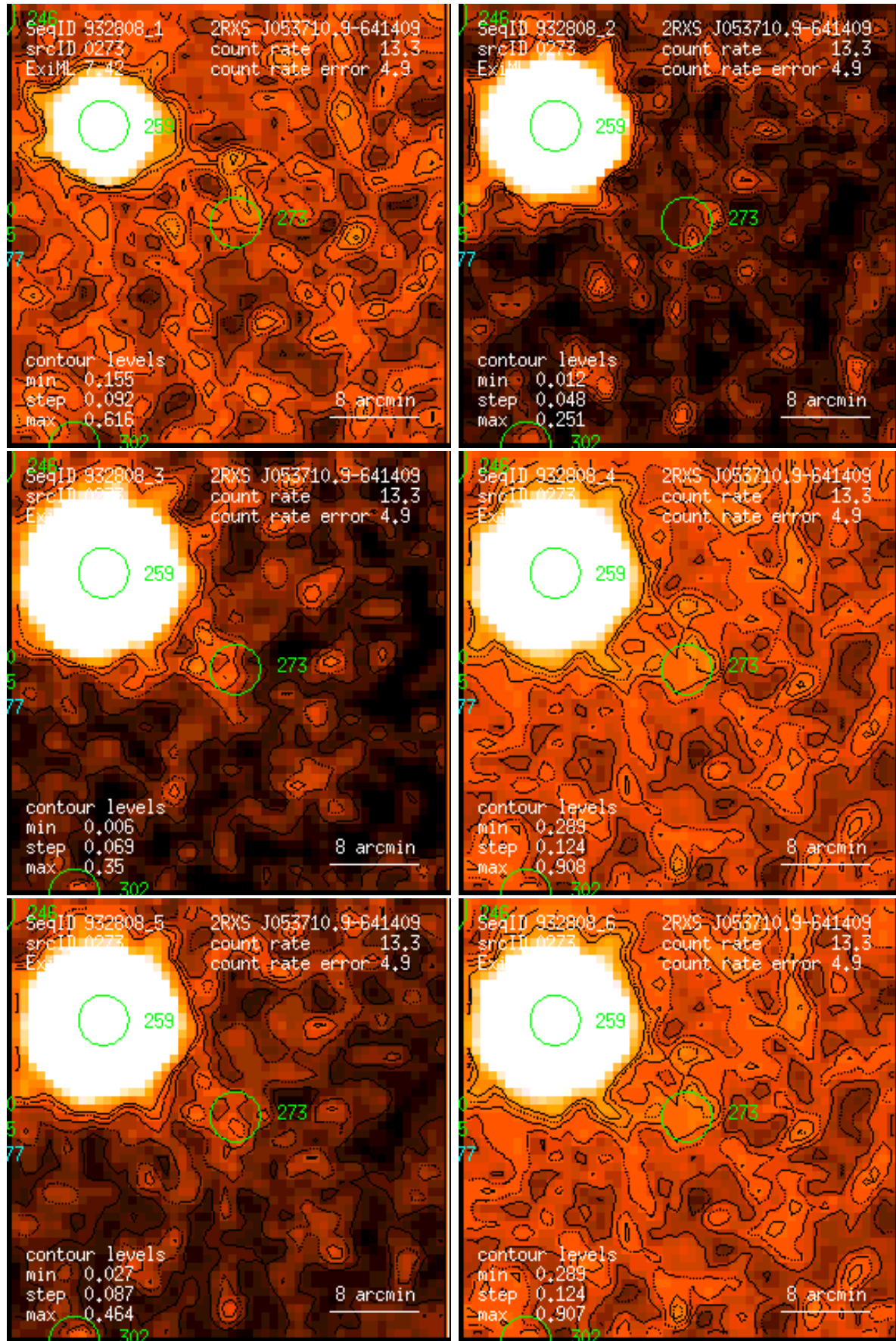
Figure 273: RASS 932808: detection 0273: band rate images, Gaussian filter: (1) PSPC channels 11 – 41, (2) 52 – 90, (3) 91 – 201, (4) 11 – 235, (5) 52 – 201, (6) 11 – 201. Broad band rates in counts/ks. Band rate contour levels in counts/ks/arcmin 2 .
