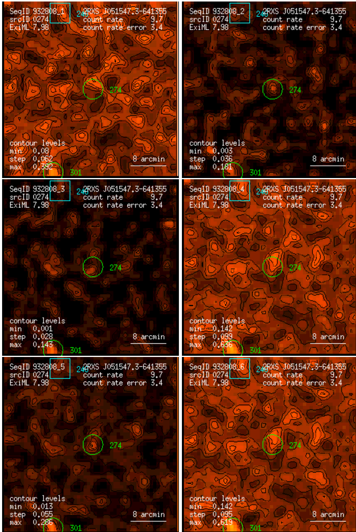
Figure 274: RASS 932808: detection 0274: band rate images, Gaussian filter: (1) PSPC channels 11 – 41, (2) 52 – 90, (3) 91 – 201, (4) 11 – 235, (5) 52 – 201, (6) 11 – 201. Broad band rates in counts/ks. Band rate contour levels in counts/ks/arcmin 2 .
