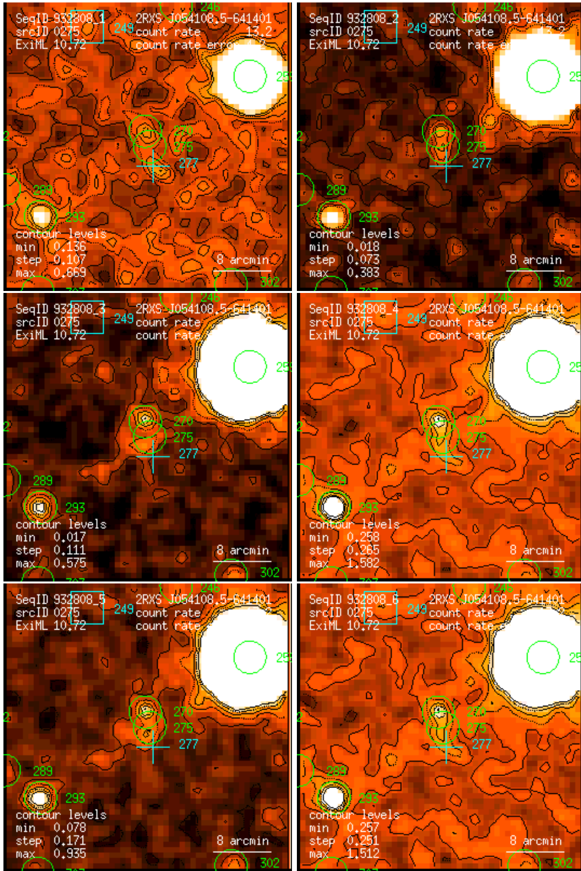
Figure 275: RASS 932808: detection 0275: band rate images, Gaussian filter: (1) PSPC channels 11 – 41, (2) 52 – 90, (3) 91 – 201, (4) 11 – 235, (5) 52 – 201, (6) 11 – 201. Broad band rates in counts/ks. Band rate contour levels in counts/ks/arcmin 2 .
