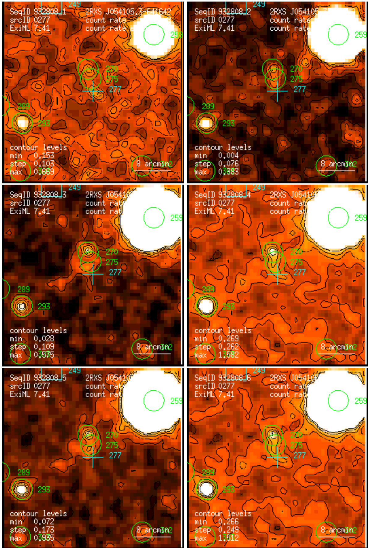
Figure 277: RASS 932808: detection 0277: band rate images, Gaussian filter: (1) PSPC channels 11 – 41, (2) 52 – 90, (3) 91 – 201, (4) 11 – 235, (5) 52 – 201, (6) 11 – 201. Broad band rates in counts/ks. Band rate contour levels in counts/ks/arcmin 2 .
