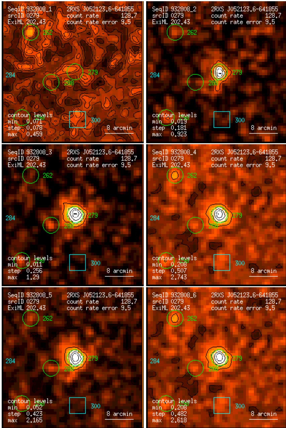
Figure 279: RASS 932808: detection 0279: band rate images, Gaussian filter: (1) PSPC channels 11 – 41, (2) 52 – 90, (3) 91 – 201, (4) 11 – 235, (5) 52 – 201, (6) 11 – 201. Broad band rates in counts/ks. Band rate contour levels in counts/ks/arcmin 2 .
