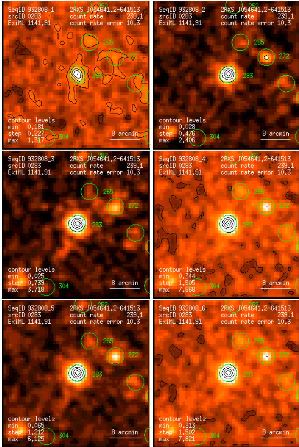
Figure 283: RASS 932808: detection 0283: band rate images, Gaussian filter: (1) PSPC channels 11 – 41, (2) 52 – 90, (3) 91 – 201, (4) 11 – 235, (5) 52 – 201, (6) 11 – 201. Broad band rates in counts/ks. Band rate contour levels in counts/ks/arcmin 2 .
