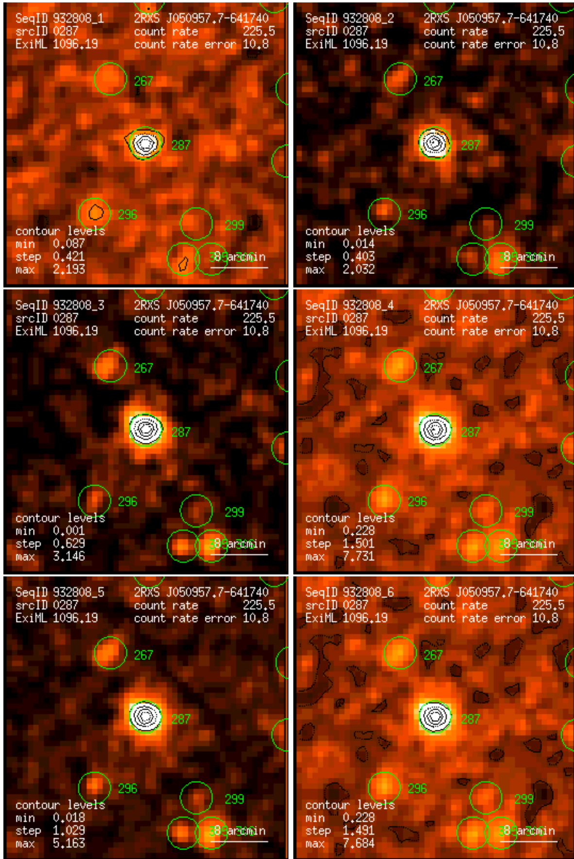
Figure 287: RASS 932808: detection 0287: band rate images, Gaussian filter: (1) PSPC channels 11 – 41, (2) 52 – 90, (3) 91 – 201, (4) 11 – 235, (5) 52 – 201, (6) 11 – 201. Broad band rates in counts/ks. Band rate contour levels in counts/ks/arcmin 2 .
