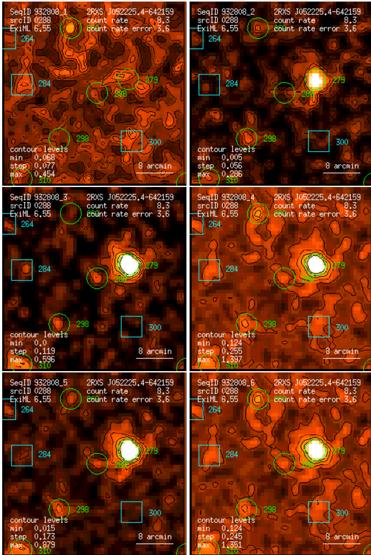
Figure 288: RASS 932808: detection 0288: band rate images, Gaussian filter: (1) PSPC channels 11 – 41, (2) 52 – 90, (3) 91 – 201, (4) 11 – 235, (5) 52 – 201, (6) 11 – 201. Broad band rates in counts/ks. Band rate contour levels in counts/ks/arcmin 2 .
