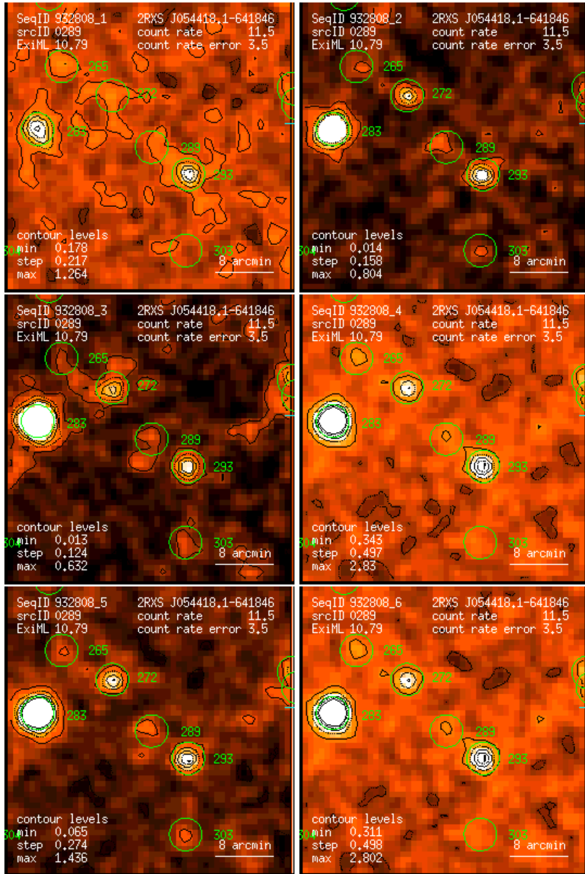
Figure 289: RASS 932808: detection 0289: band rate images, Gaussian filter: (1) PSPC channels 11 – 41, (2) 52 – 90, (3) 91 – 201, (4) 11 – 235, (5) 52 – 201, (6) 11 – 201. Broad band rates in counts/ks. Band rate contour levels in counts/ks/arcmin 2 .
