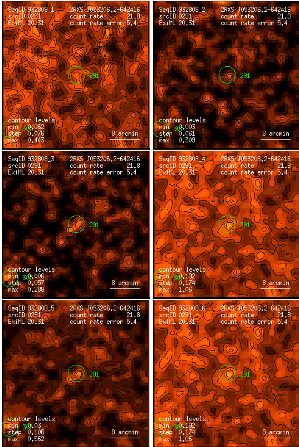
Figure 291: RASS 932808: detection 0291: band rate images, Gaussian filter: (1) PSPC channels 11 – 41, (2) 52 – 90, (3) 91 – 201, (4) 11 – 235, (5) 52 – 201, (6) 11 – 201. Broad band rates in counts/ks. Band rate contour levels in counts/ks/arcmin 2 .
