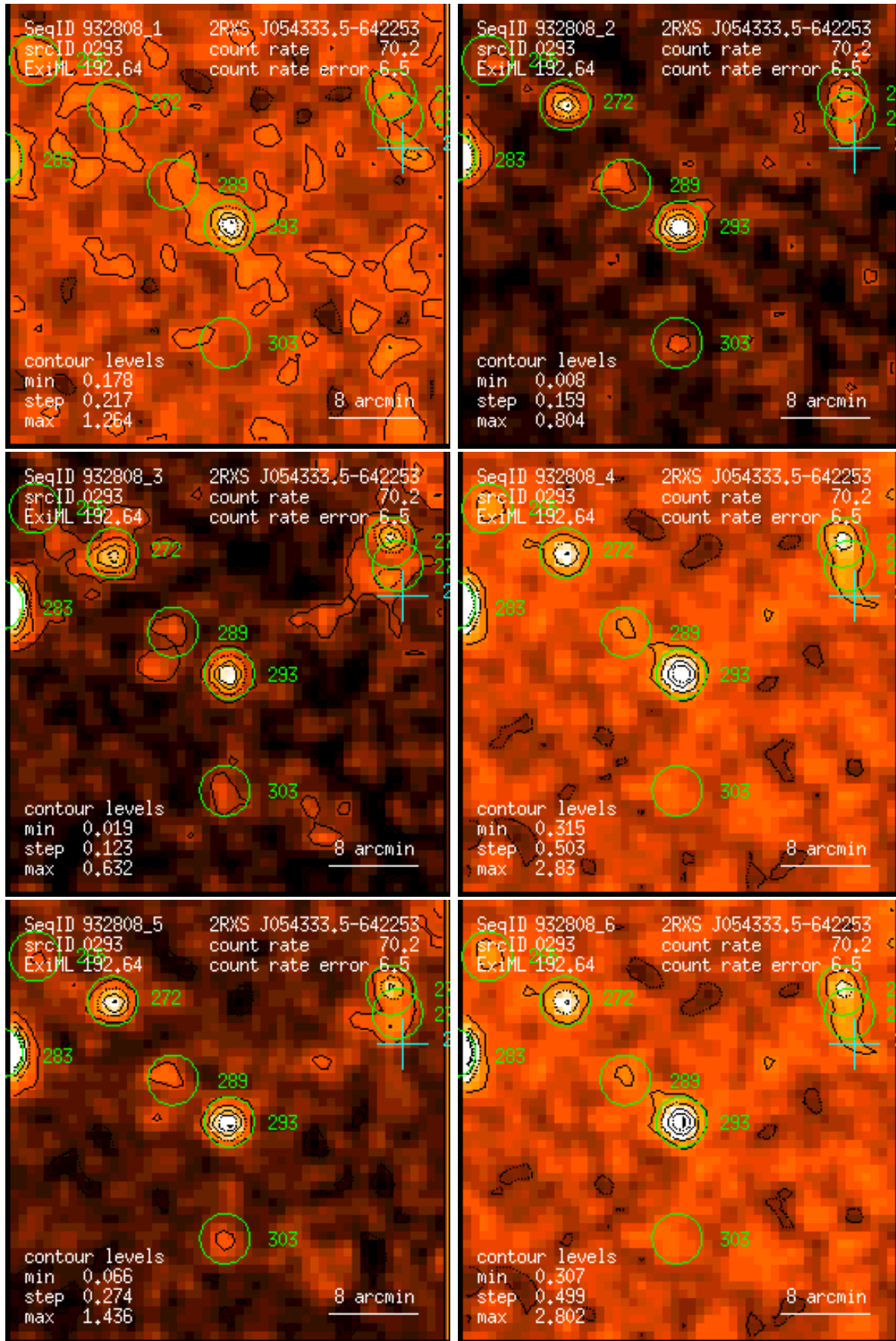
Figure 293: RASS 932808: detection 0293: band rate images, Gaussian filter: (1) PSPC channels 11 – 41, (2) 52 – 90, (3) 91 – 201, (4) 11 – 235, (5) 52 – 201, (6) 11 – 201. Broad band rates in counts/ks. Band rate contour levels in counts/ks/arcmin 2 .
