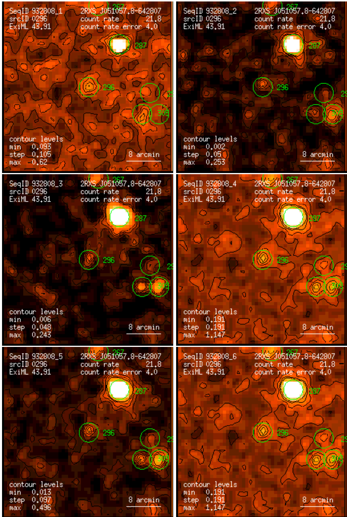
Figure 296: RASS 932808: detection 0296: band rate images, Gaussian filter: (1) PSPC channels 11 – 41, (2) 52 – 90, (3) 91 – 201, (4) 11 – 235, (5) 52 – 201, (6) 11 – 201. Broad band rates in counts/ks. Band rate contour levels in counts/ks/arcmin 2 .
