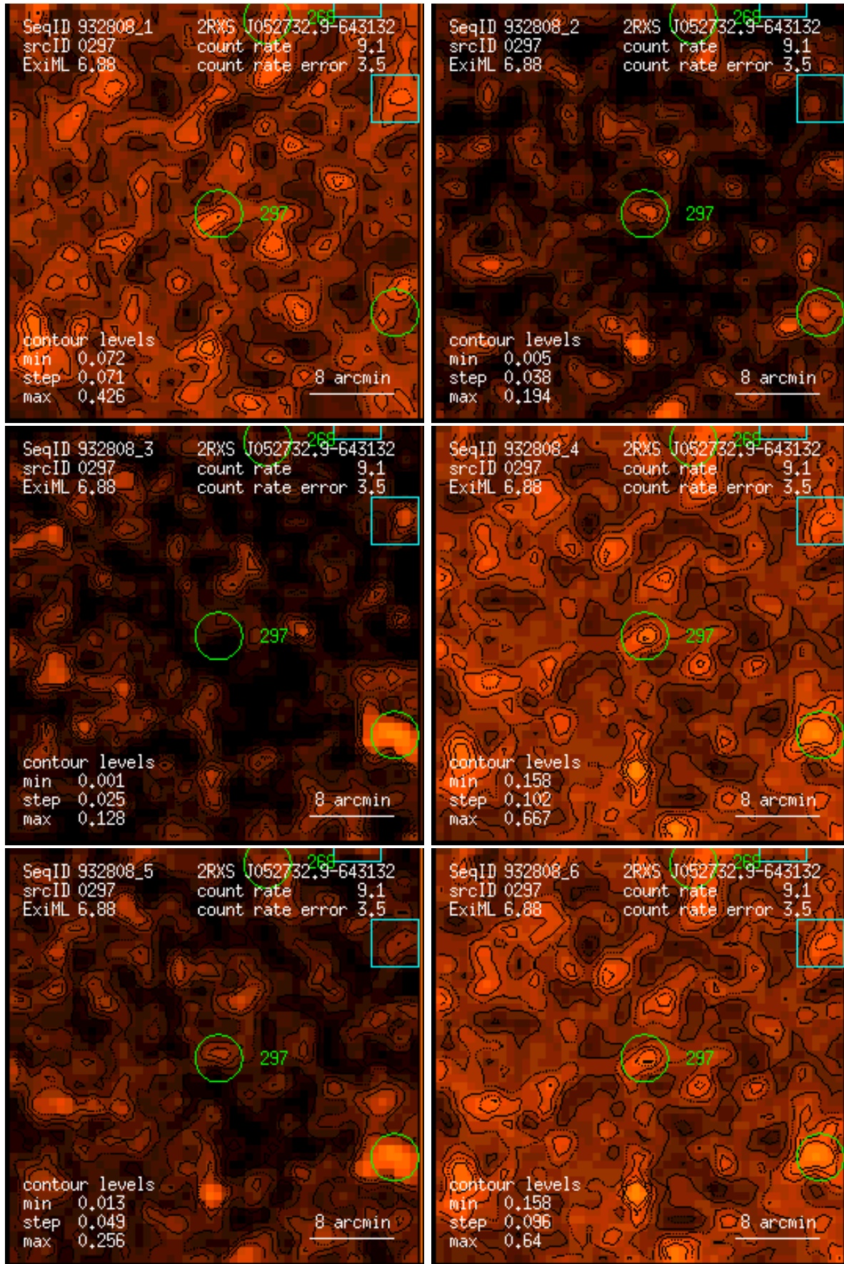
Figure 297: RASS 932808: detection 0297: band rate images, Gaussian filter: (1) PSPC channels 11 – 41, (2) 52 – 90, (3) 91 – 201, (4) 11 – 235, (5) 52 – 201, (6) 11 – 201. Broad band rates in counts/ks. Band rate contour levels in counts/ks/arcmin 2 .
