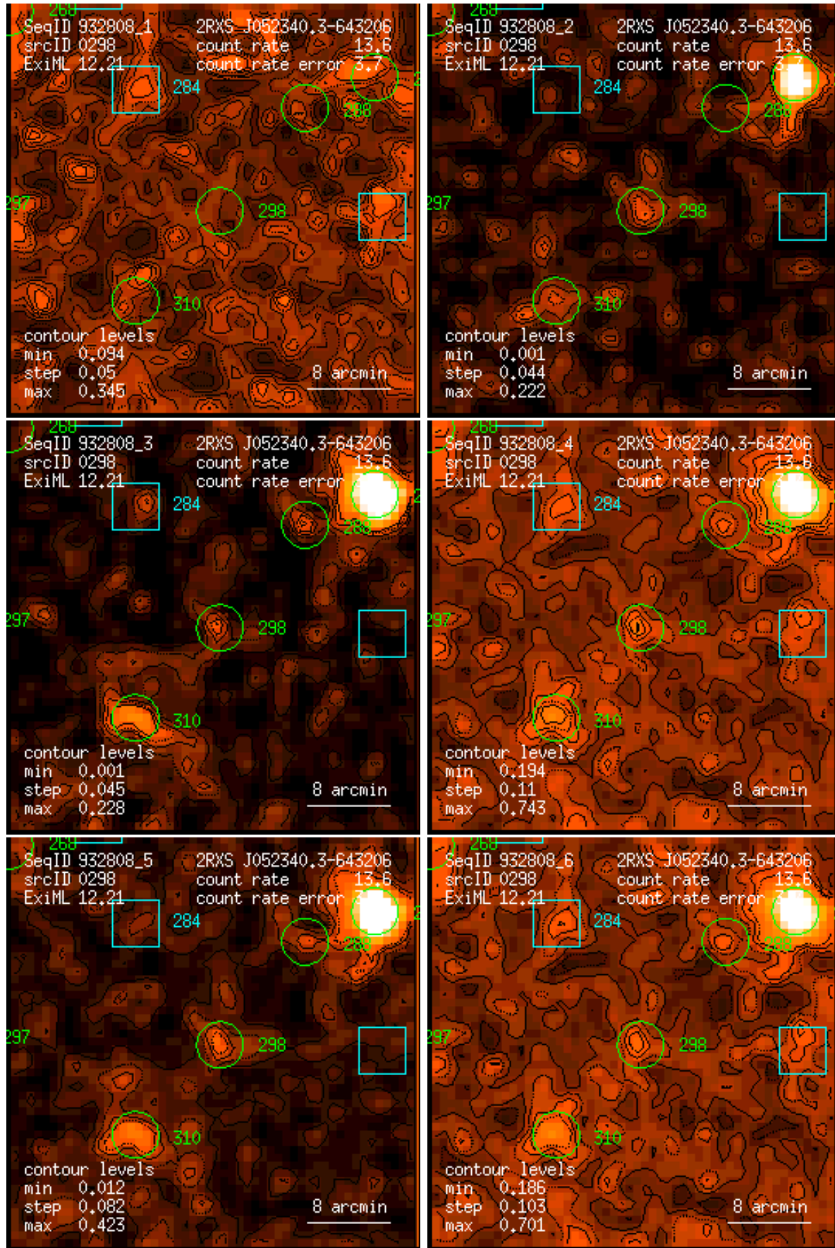
Figure 298: RASS 932808: detection 0298: band rate images, Gaussian filter: (1) PSPC channels 11 – 41, (2) 52 – 90, (3) 91 – 201, (4) 11 – 235, (5) 52 – 201, (6) 11 – 201. Broad band rates in counts/ks. Band rate contour levels in counts/ks/arcmin 2 .
