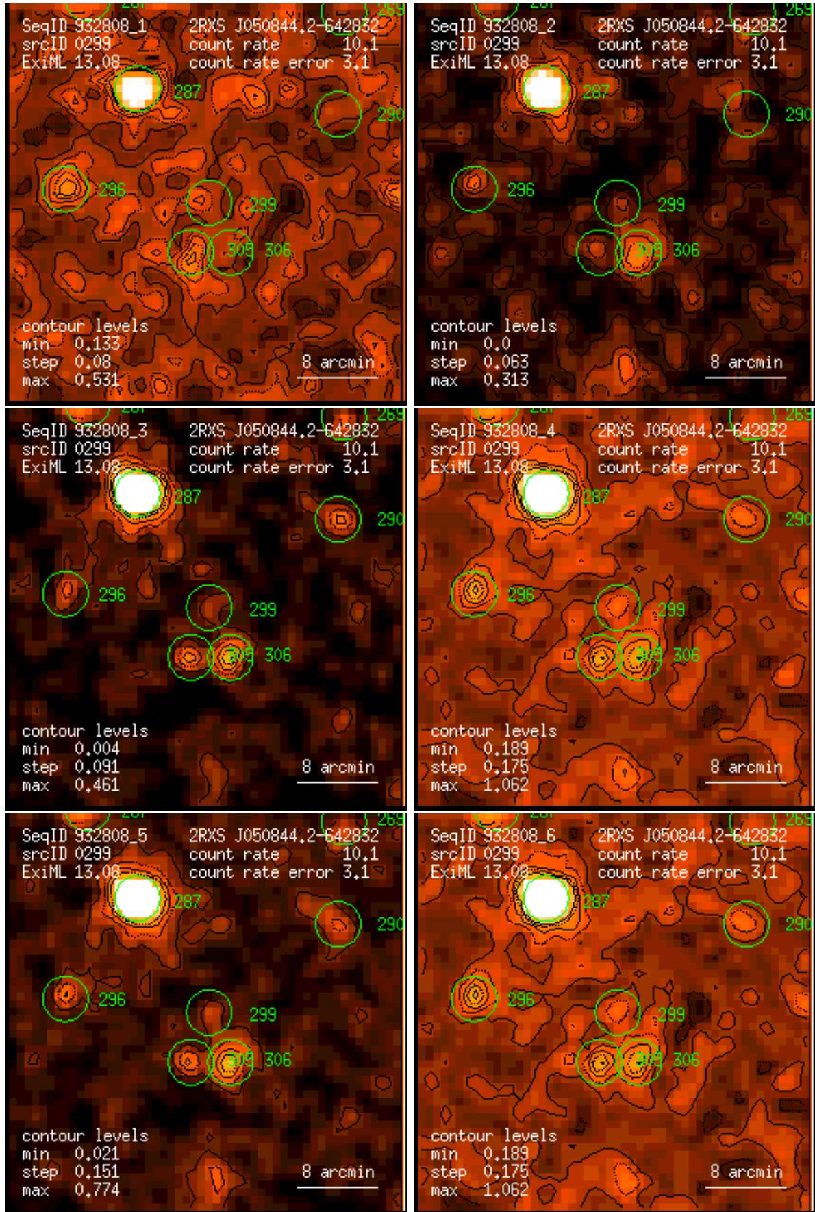
Figure 299: RASS 932808: detection 0299: band rate images, Gaussian filter: (1) PSPC channels 11 – 41, (2) 52 – 90, (3) 91 – 201, (4) 11 – 235, (5) 52 – 201, (6) 11 – 201. Broad band rates in counts/ks. Band rate contour levels in counts/ks/arcmin 2 .
