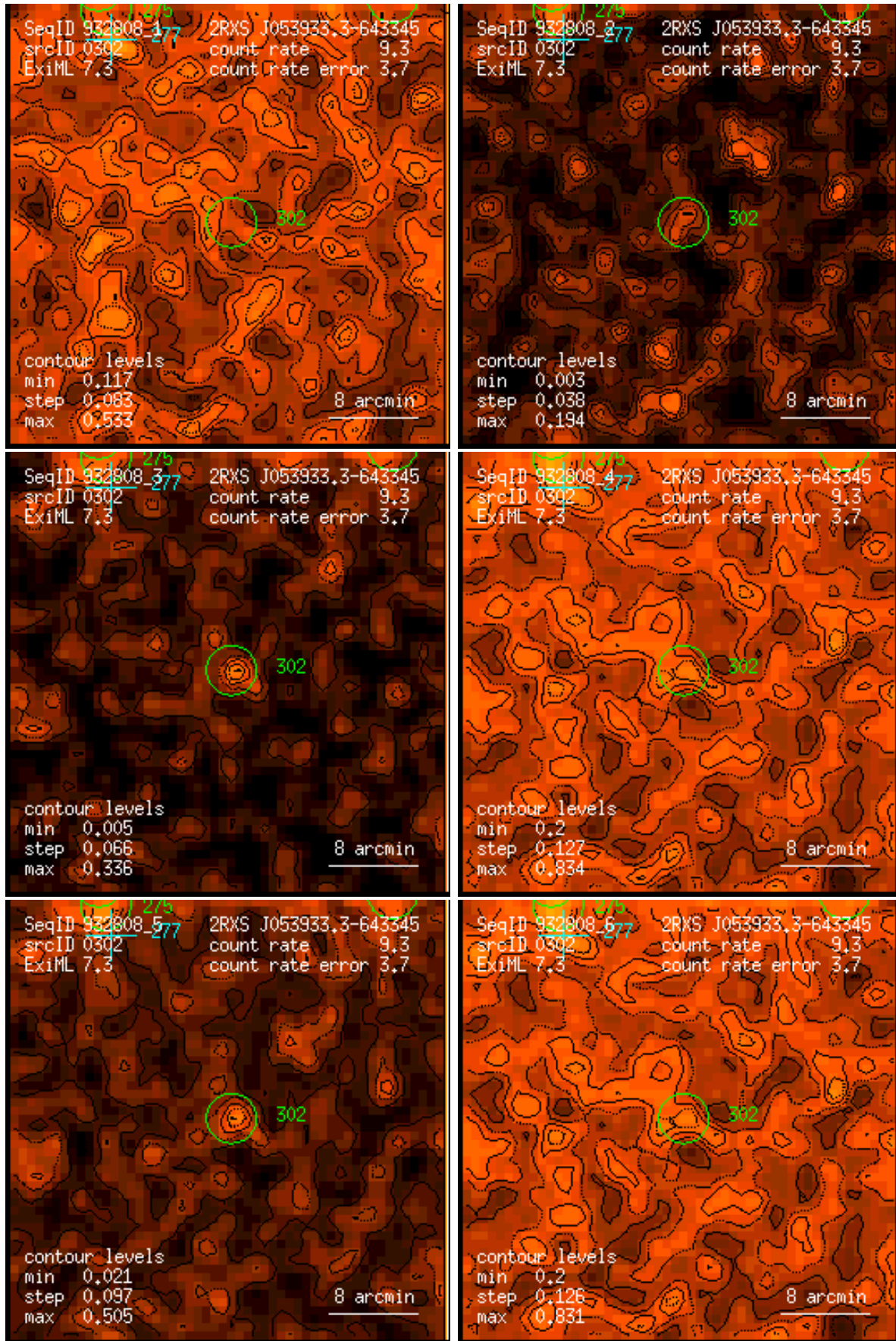
Figure 302: RASS 932808: detection 0302: band rate images, Gaussian filter: (1) PSPC channels 11 – 41, (2) 52 – 90, (3) 91 – 201, (4) 11 – 235, (5) 52 – 201, (6) 11 – 201. Broad band rates in counts/ks. Band rate contour levels in counts/ks/arcmin 2 .
