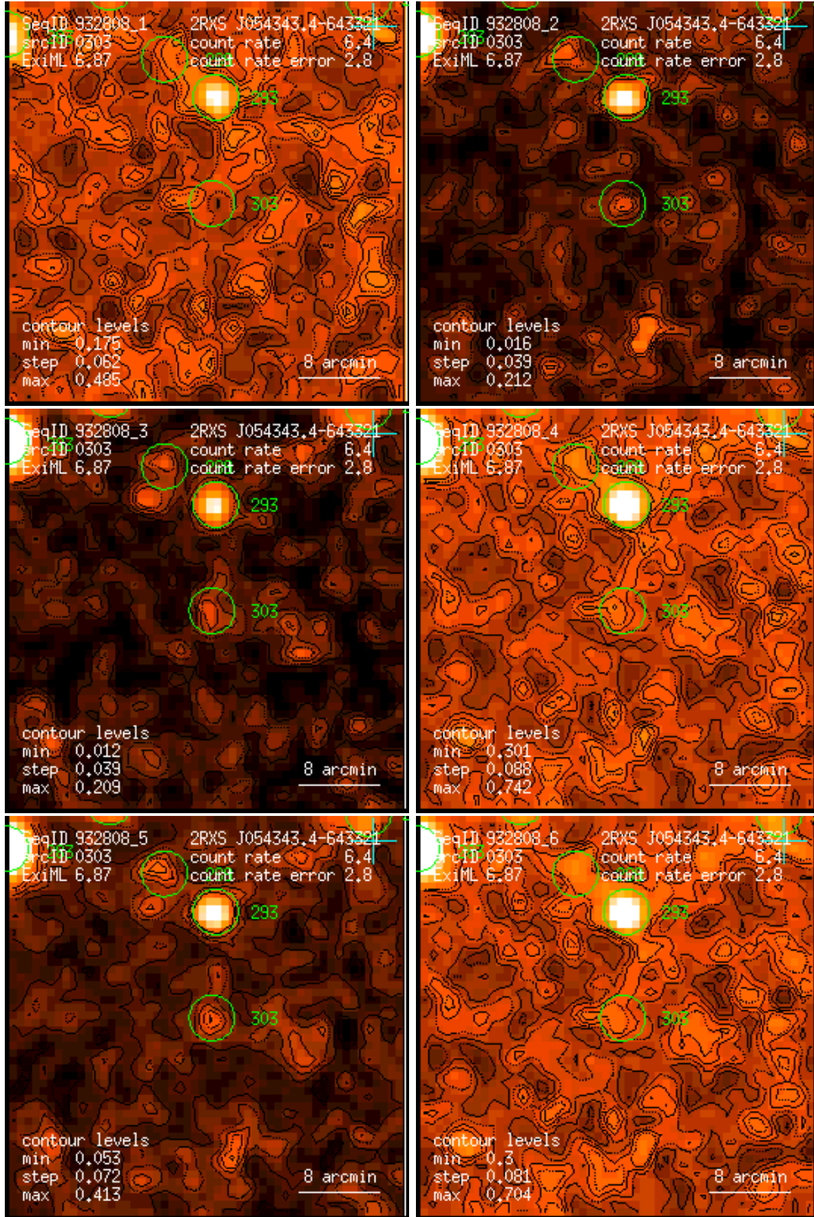
Figure 303: RASS 932808: detection 0303: band rate images, Gaussian filter: (1) PSPC channels 11 – 41, (2) 52 – 90, (3) 91 – 201, (4) 11 – 235, (5) 52 – 201, (6) 11 – 201. Broad band rates in counts/ks. Band rate contour levels in counts/ks/arcmin 2 .
