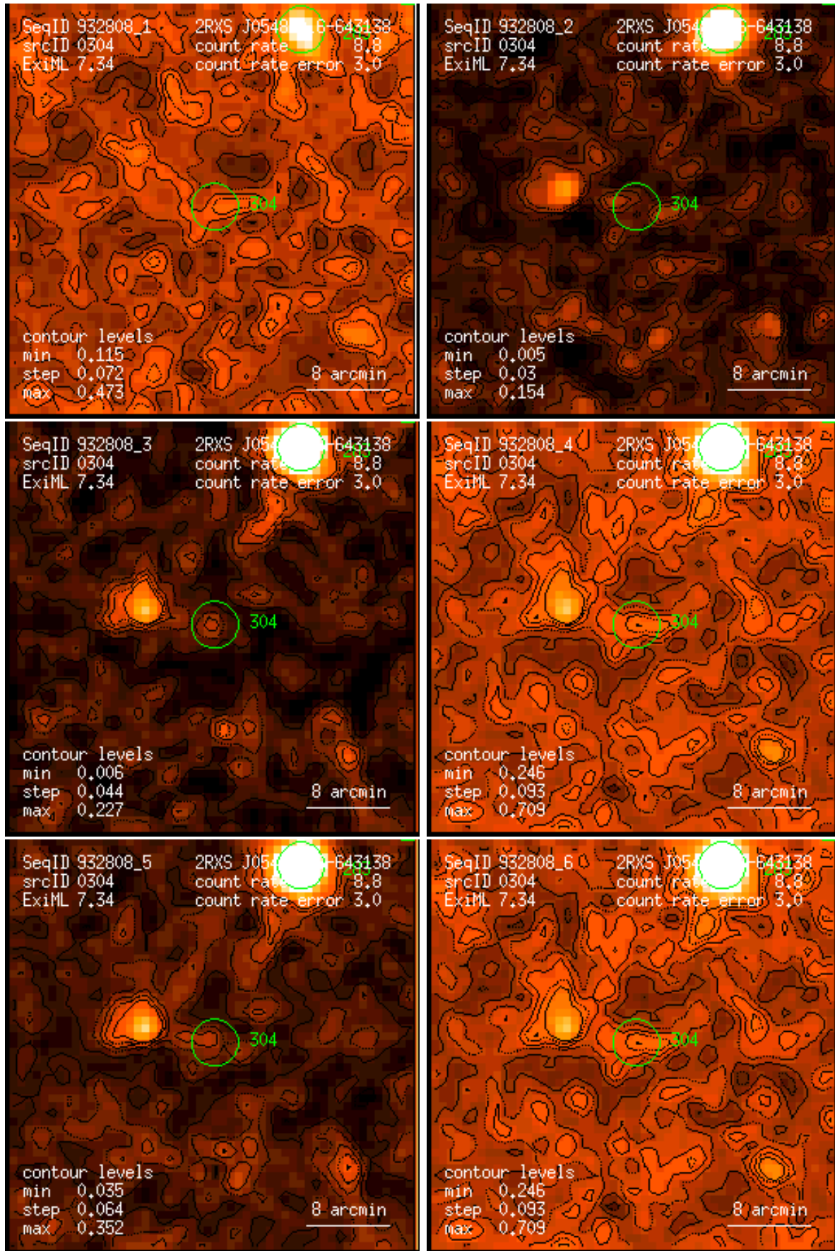
Figure 304: RASS 932808: detection 0304: band rate images, Gaussian filter: (1) PSPC channels 11 – 41, (2) 52 – 90, (3) 91 – 201, (4) 11 – 235, (5) 52 – 201, (6) 11 – 201. Broad band rates in counts/ks. Band rate contour levels in counts/ks/arcmin 2 .
