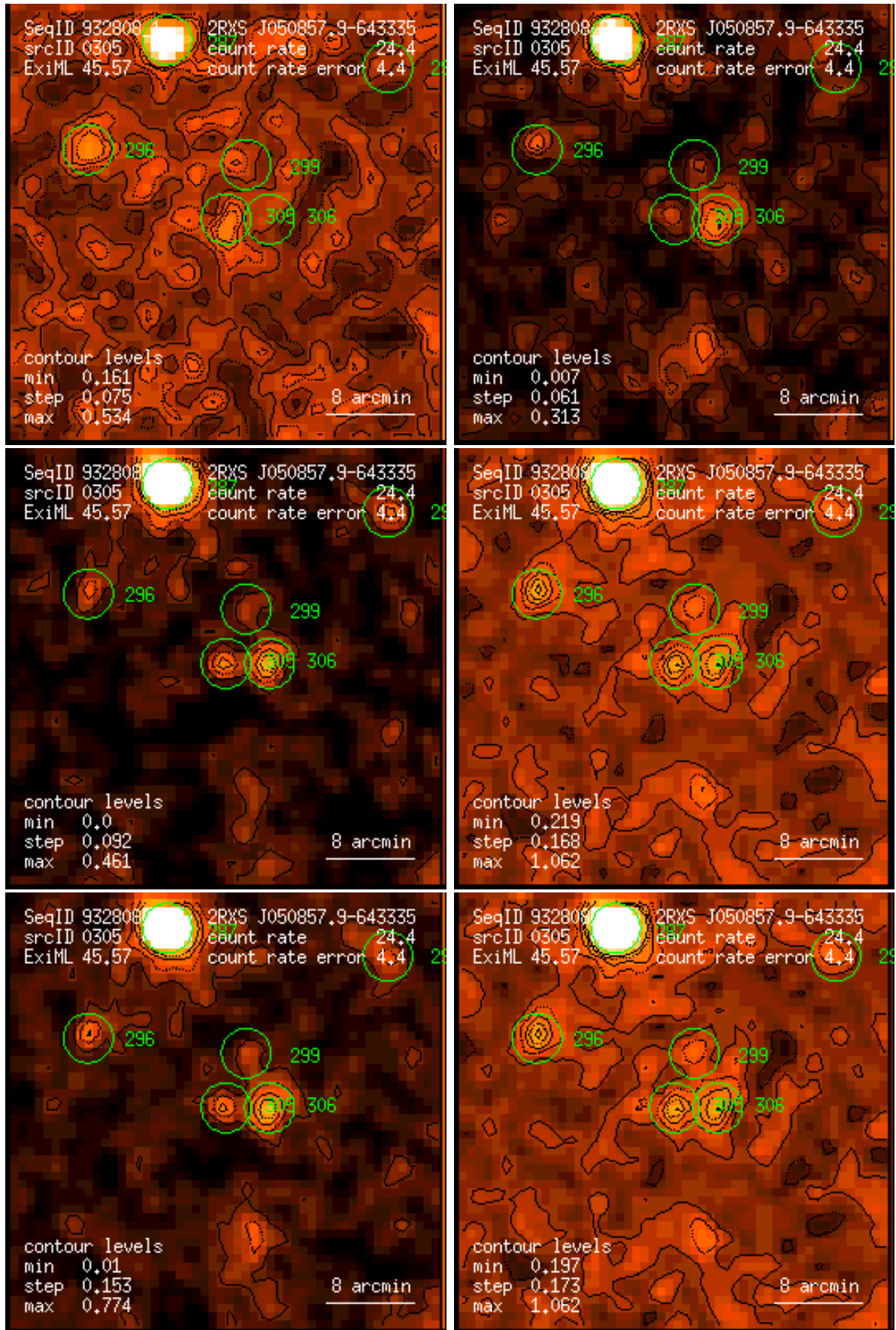
Figure 305: RASS 932808: detection 0305: band rate images, Gaussian filter: (1) PSPC channels 11 – 41, (2) 52 – 90, (3) 91 – 201, (4) 11 – 235, (5) 52 – 201, (6) 11 – 201. Broad band rates in counts/ks. Band rate contour levels in counts/ks/arcmin 2 .
