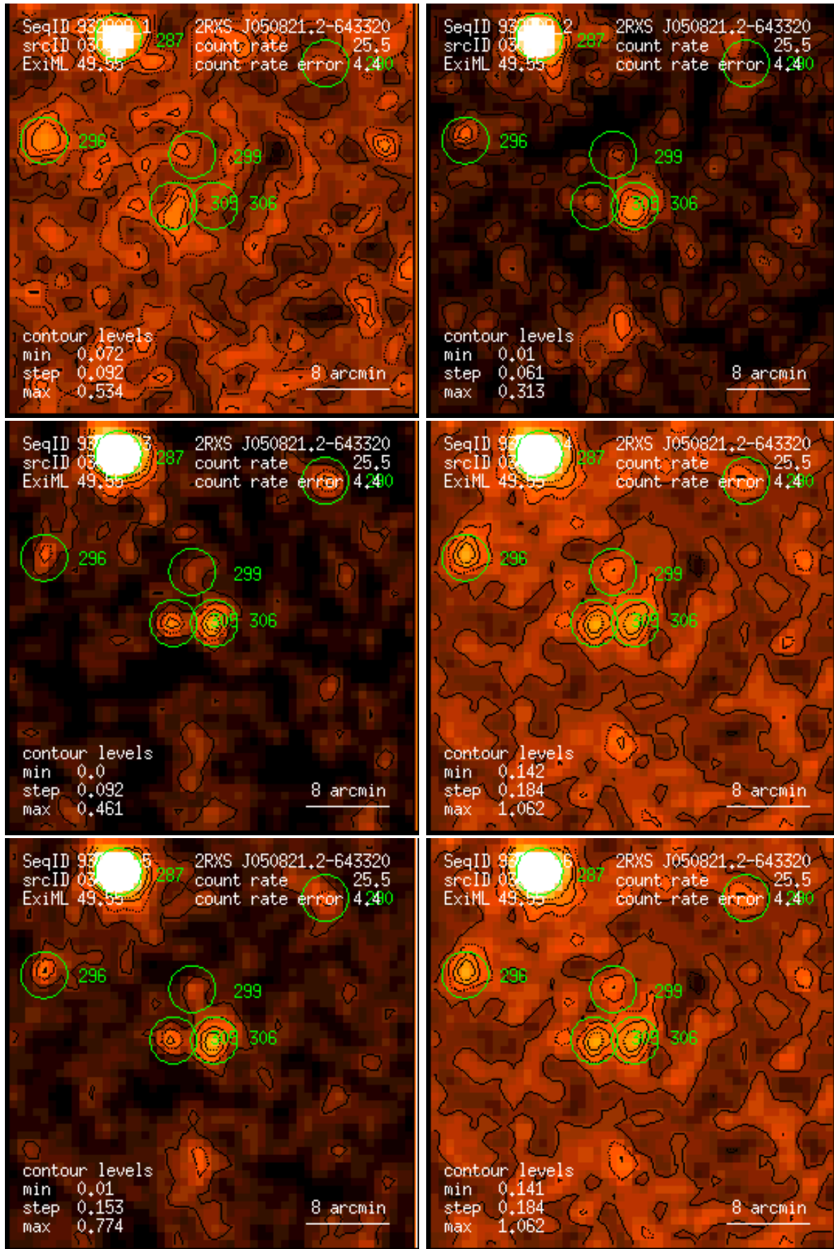
Figure 306: RASS 932808: detection 0306: band rate images, Gaussian filter: (1) PSPC channels 11 – 41, (2) 52 – 90, (3) 91 – 201, (4) 11 – 235, (5) 52 – 201, (6) 11 – 201. Broad band rates in counts/ks. Band rate contour levels in counts/ks/arcmin 2 .
