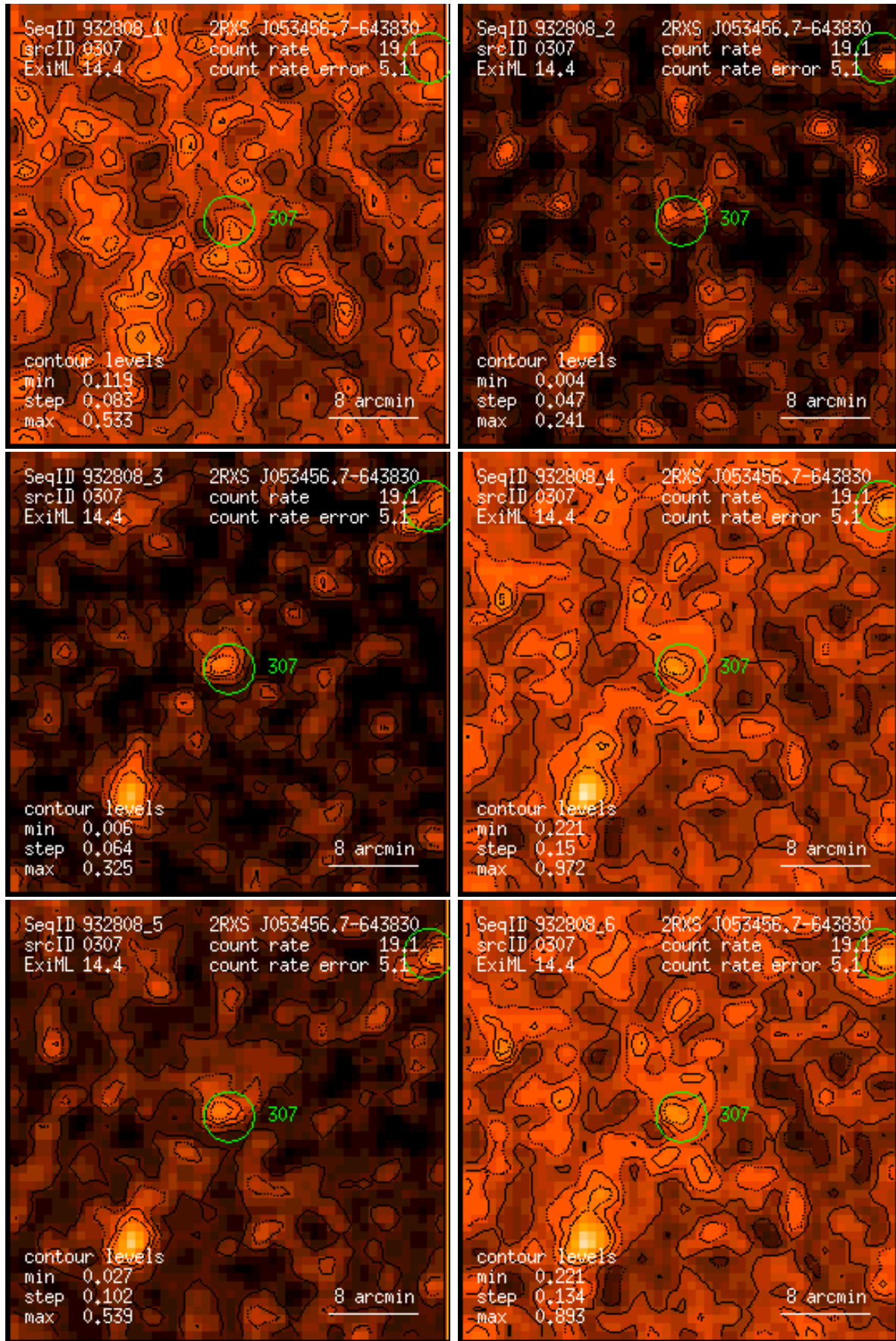
Figure 307: RASS 932808: detection 0307: band rate images, Gaussian filter: (1) PSPC channels 11 – 41, (2) 52 – 90, (3) 91 – 201, (4) 11 – 235, (5) 52 – 201, (6) 11 – 201. Broad band rates in counts/ks. Band rate contour levels in counts/ks/arcmin 2 .
