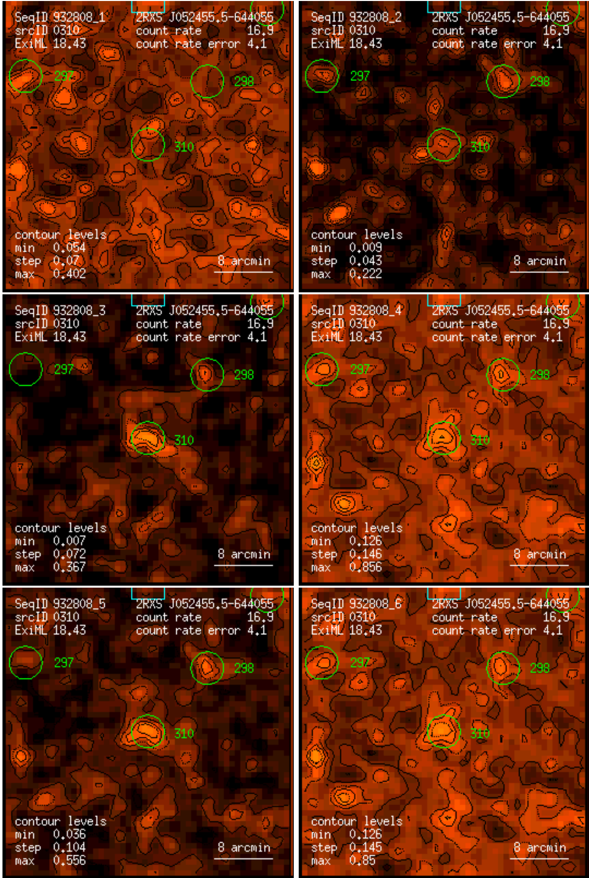
Figure 310: RASS 932808: detection 0310: band rate images, Gaussian filter: (1) PSPC channels 11 – 41, (2) 52 – 90, (3) 91 – 201, (4) 11 – 235, (5) 52 – 201, (6) 11 – 201. Broad band rates in counts/ks. Band rate contour levels in counts/ks/arcmin 2 .
