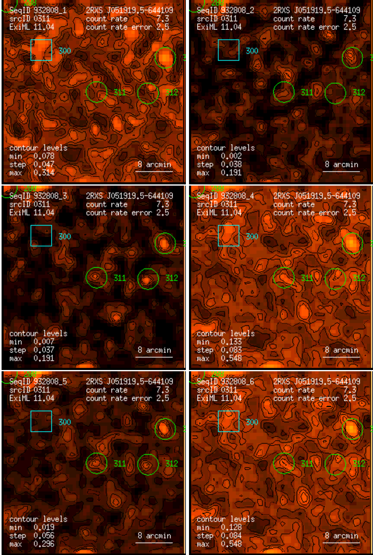
Figure 311: RASS 932808: detection 0311: band rate images, Gaussian filter: (1) PSPC channels 11 – 41, (2) 52 – 90, (3) 91 – 201, (4) 11 – 235, (5) 52 – 201, (6) 11 – 201. Broad band rates in counts/ks. Band rate contour levels in counts/ks/arcmin 2 .
