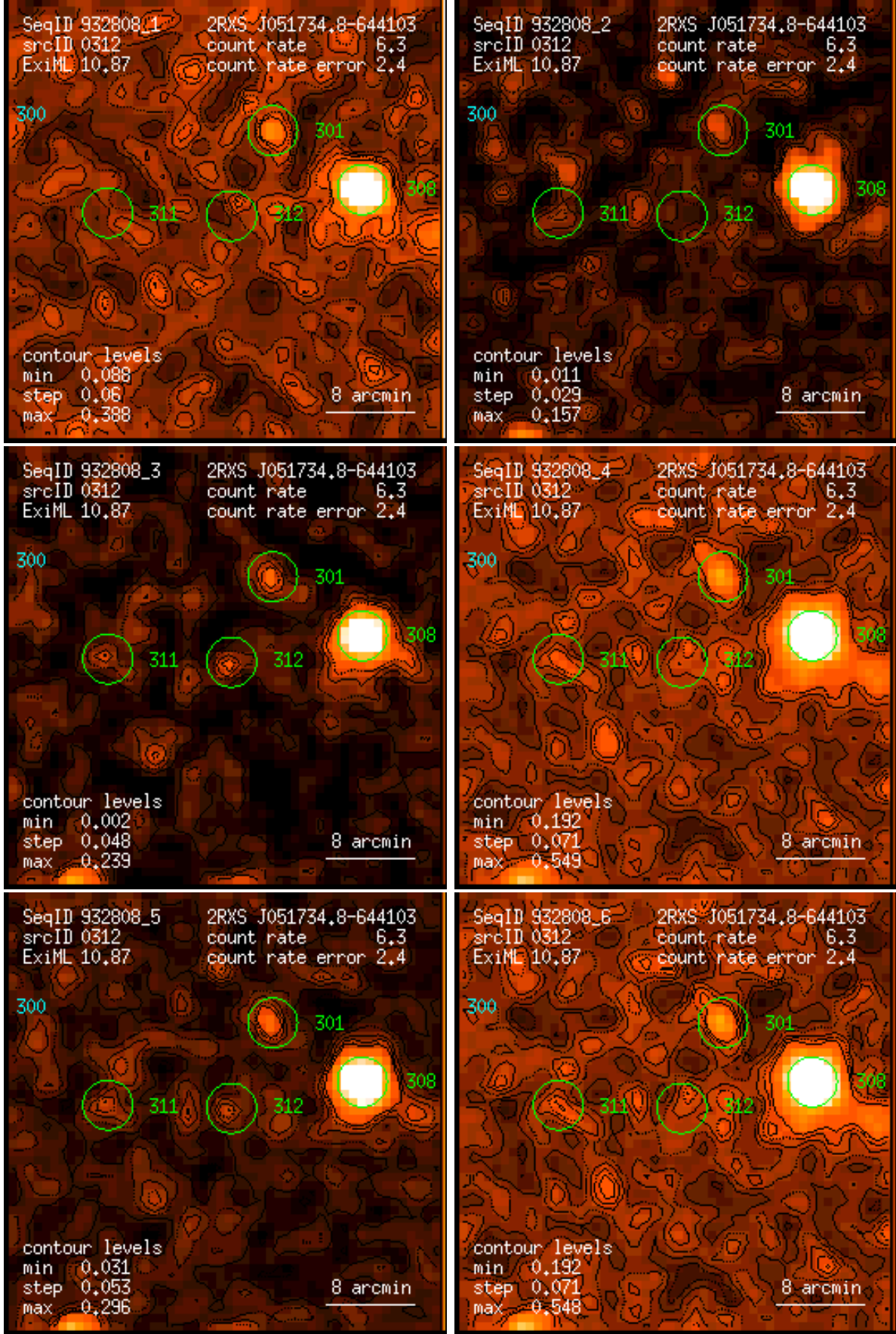
Figure 312: RASS 932808: detection 0312: band rate images, Gaussian filter: (1) PSPC channels 11 – 41, (2) 52 – 90, (3) 91 – 201, (4) 11 – 235, (5) 52 – 201, (6) 11 – 201. Broad band rates in counts/ks. Band rate contour levels in counts/ks/arcmin 2 .
