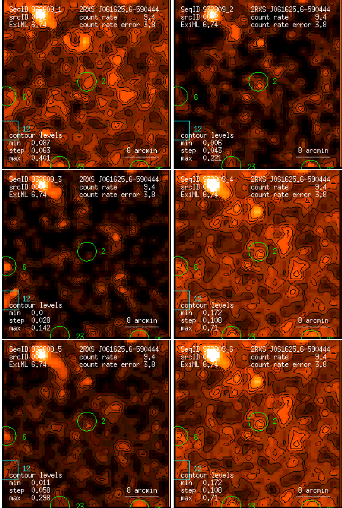
Figure 2: RASS 932809: detection 0002: band rate images, Gaussian filter: (1) PSPC channels 11 – 41, (2) 52 – 90, (3) 91 – 201, (4) 11 – 235, (5) 52 – 201, (6) 11 – 201. Broad band rates in counts/ks. Band rate contour levels in counts/ks/arcmin 2 .
