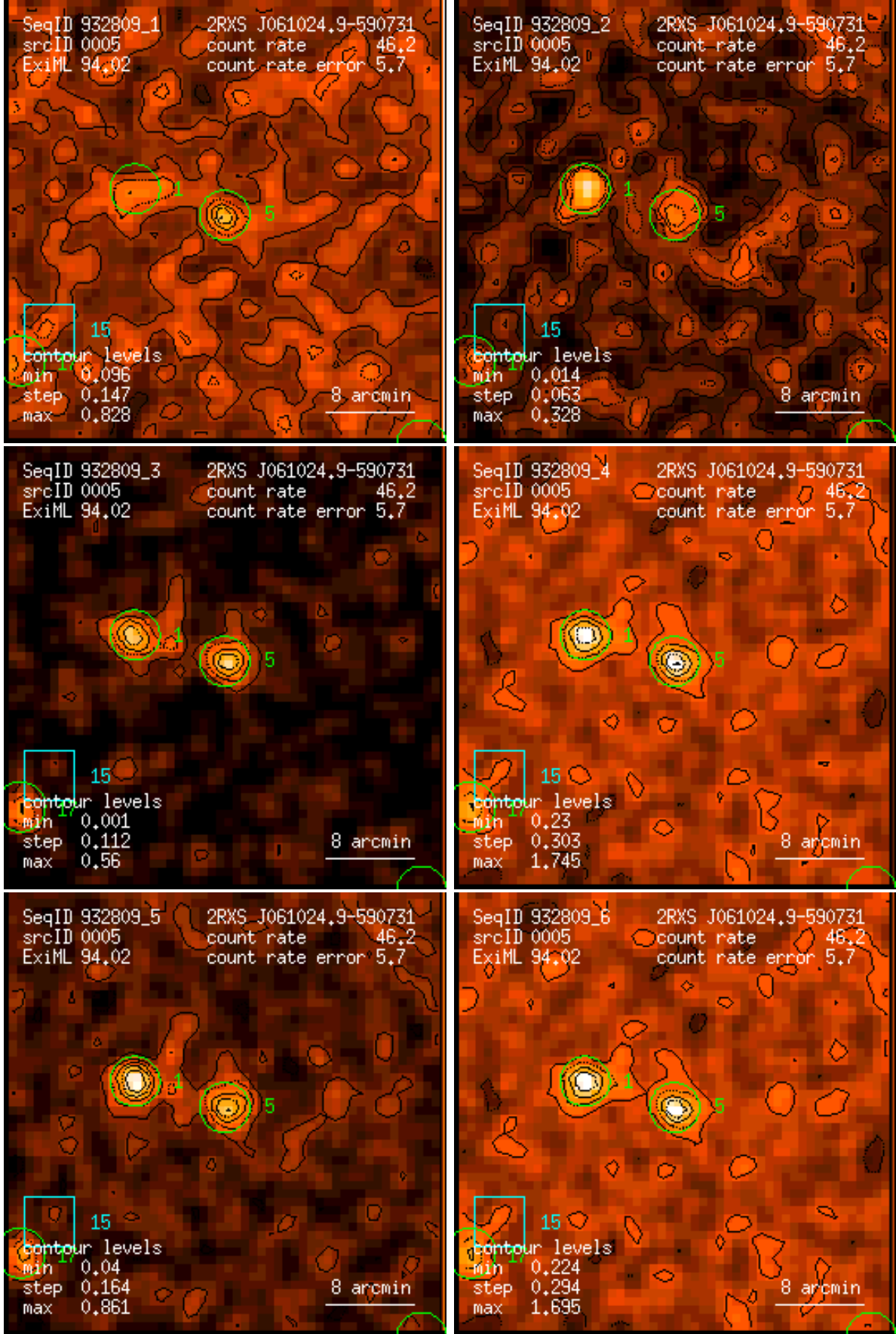
Figure 5: RASS 932809: detection 0005: band rate images, Gaussian filter: (1) PSPC channels 11 – 41, (2) 52 – 90, (3) 91 – 201, (4) 11 – 235, (5) 52 – 201, (6) 11 – 201. Broad band rates in counts/ks. Band rate contour levels in counts/ks/arcmin 2 .
