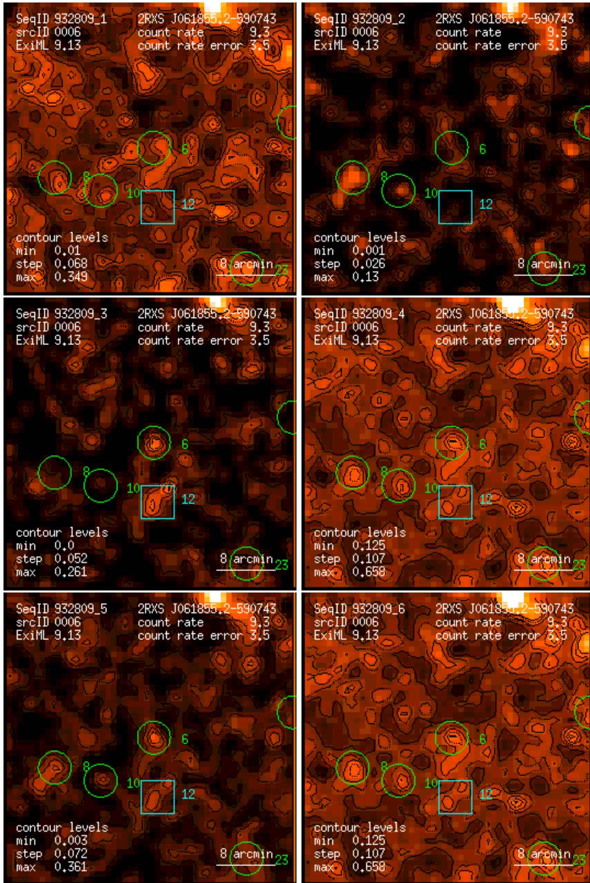
Figure 6: RASS 932809: detection 0006: band rate images, Gaussian filter: (1) PSPC channels 11 – 41, (2) 52 – 90, (3) 91 – 201, (4) 11 – 235, (5) 52 – 201, (6) 11 – 201. Broad band rates in counts/ks. Band rate contour levels in counts/ks/arcmin 2 .
