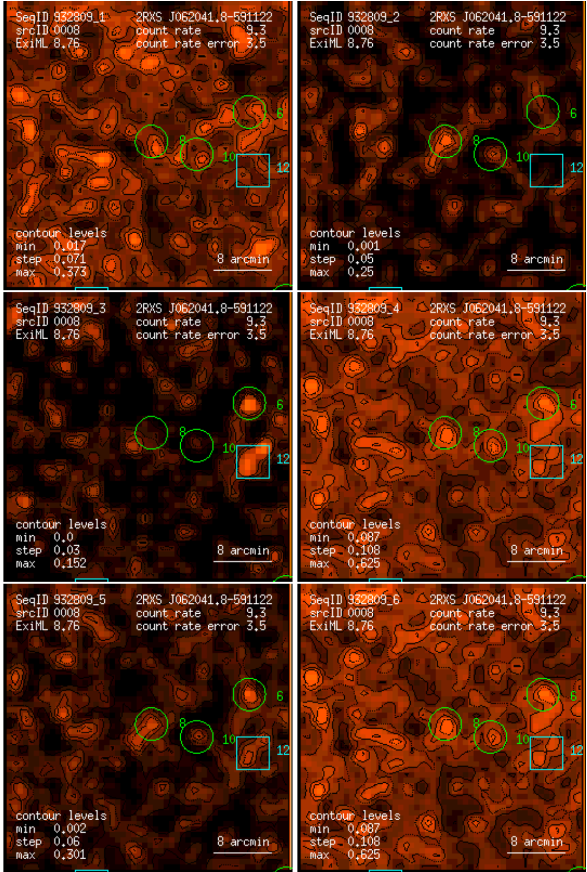
Figure 8: RASS 932809: detection 0008: band rate images, Gaussian filter: (1) PSPC channels 11 – 41, (2) 52 – 90, (3) 91 – 201, (4) 11 – 235, (5) 52 – 201, (6) 11 – 201. Broad band rates in counts/ks. Band rate contour levels in counts/ks/arcmin 2 .
