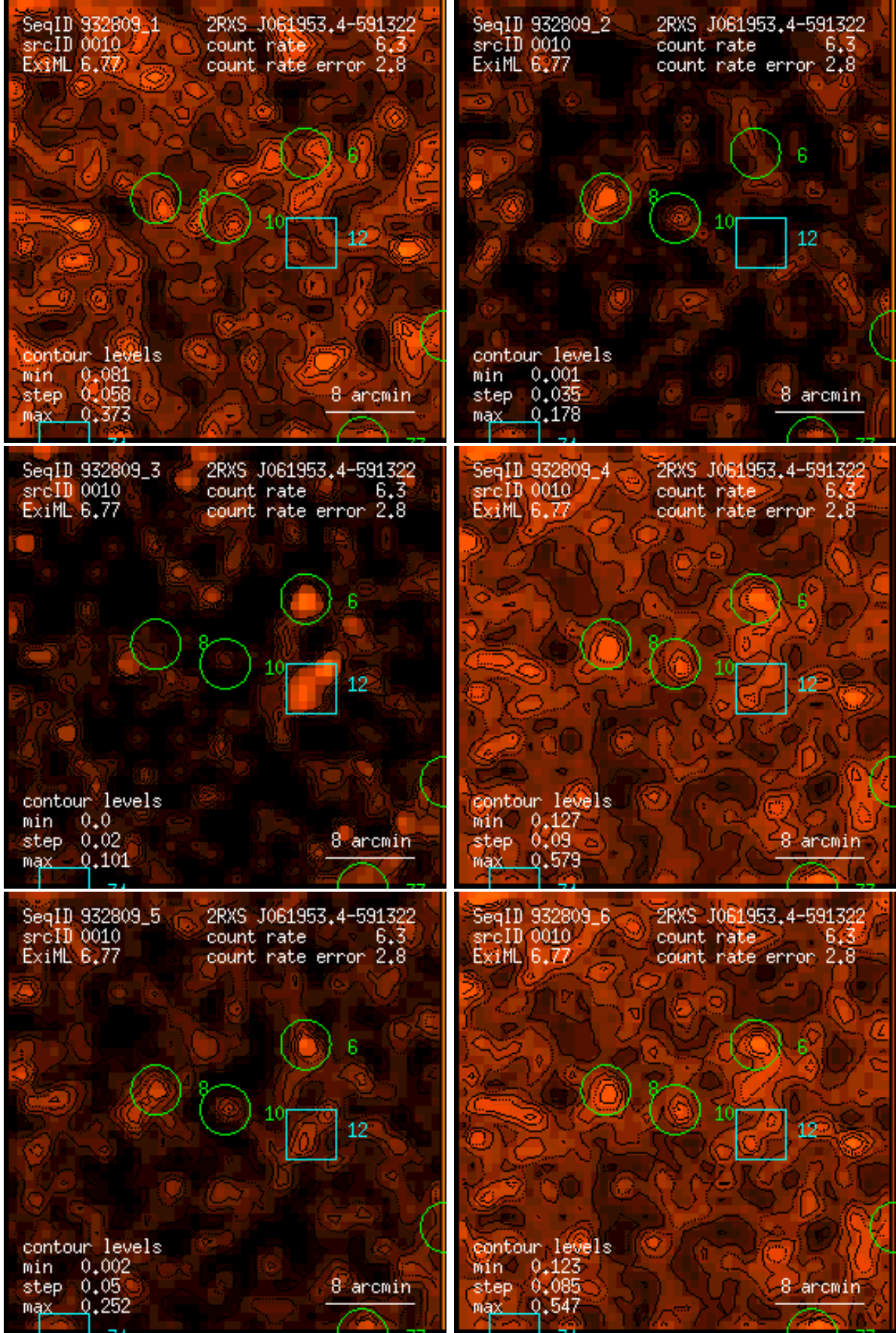
Figure 10: RASS 932809: detection 0010: band rate images, Gaussian filter: (1) PSPC channels 11 – 41, (2) 52 – 90, (3) 91 – 201, (4) 11 – 235, (5) 52 – 201, (6) 11 – 201. Broad band rates in counts/ks. Band rate contour levels in counts/ks/arcmin 2 .
