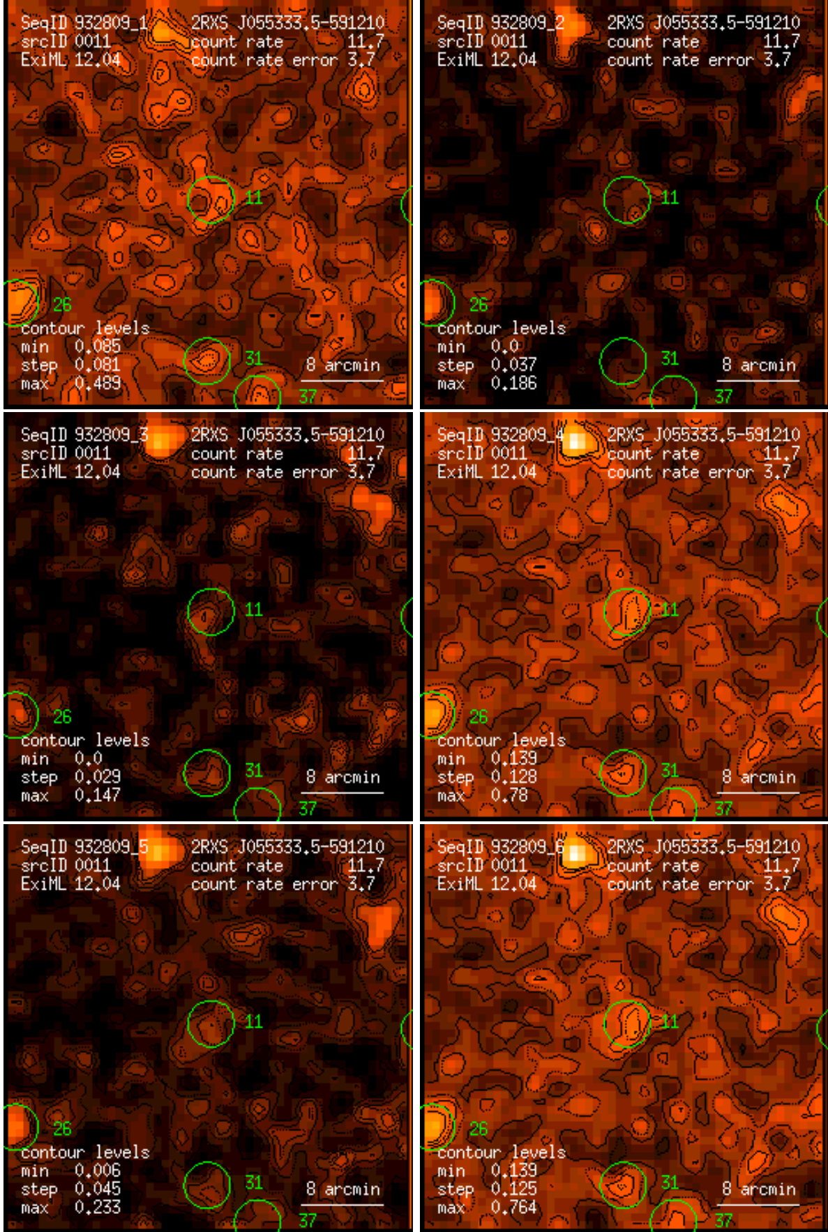
Figure 11: RASS 932809: detection 0011: band rate images, Gaussian filter: (1) PSPC channels 11 – 41, (2) 52 – 90, (3) 91 – 201, (4) 11 – 235, (5) 52 – 201, (6) 11 – 201. Broad band rates in counts/ks. Band rate contour levels in counts/ks/arcmin 2 .
