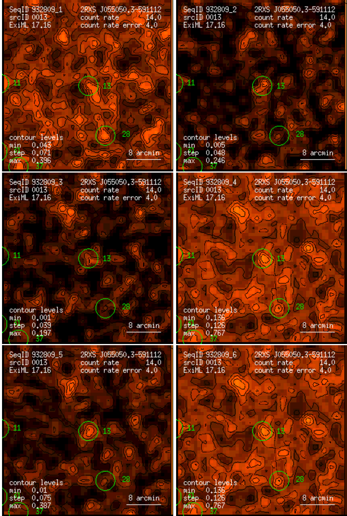
Figure 13: RASS 932809: detection 0013: band rate images, Gaussian filter: (1) PSPC channels 11 – 41, (2) 52 – 90, (3) 91 – 201, (4) 11 – 235, (5) 52 – 201, (6) 11 – 201. Broad band rates in counts/ks. Band rate contour levels in counts/ks/arcmin 2 .
