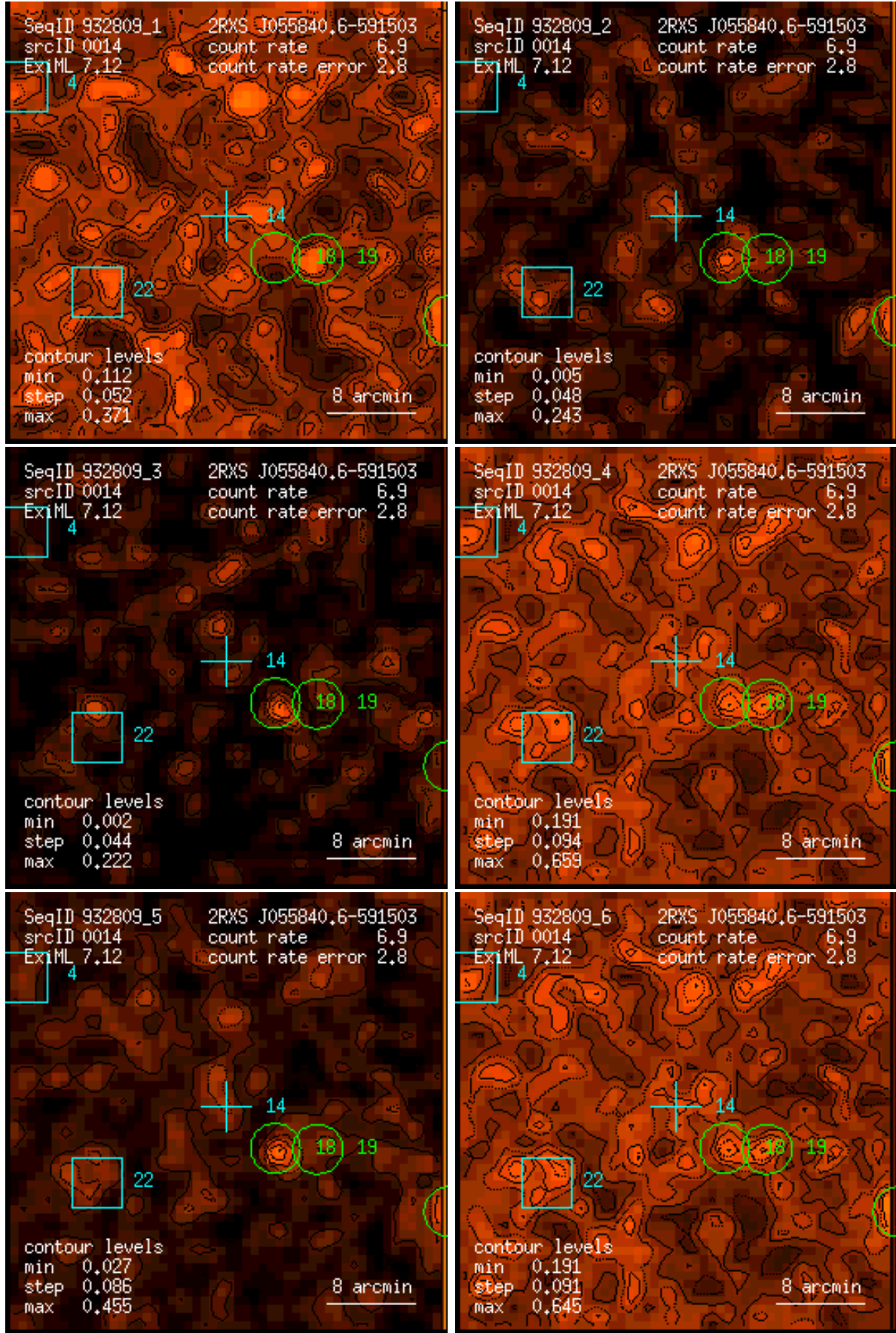
Figure 14: RASS 932809: detection 0014: band rate images, Gaussian filter: (1) PSPC channels 11 – 41, (2) 52 – 90, (3) 91 – 201, (4) 11 – 235, (5) 52 – 201, (6) 11 – 201. Broad band rates in counts/ks. Band rate contour levels in counts/ks/arcmin 2 .
