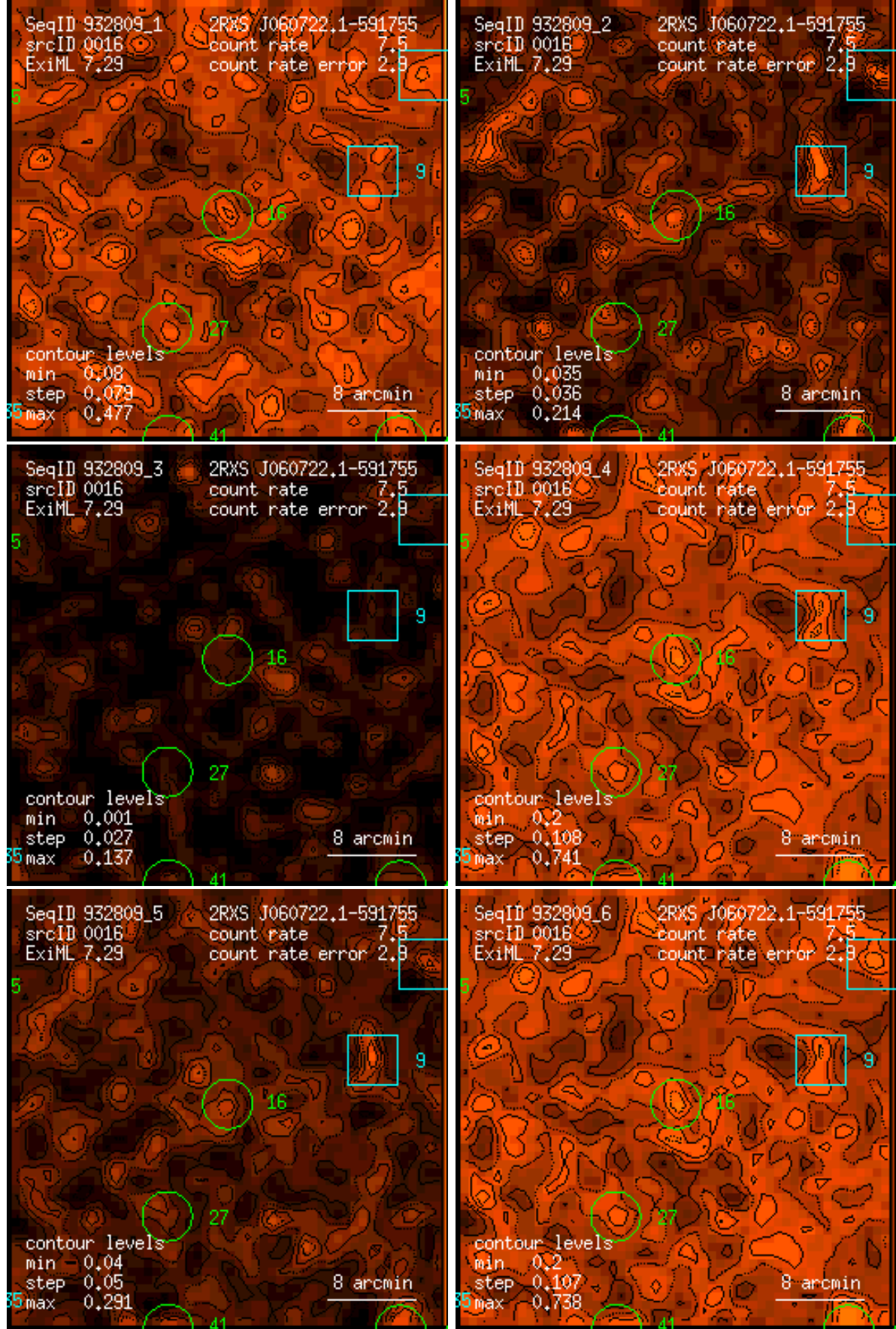
Figure 16: RASS 932809: detection 0016: band rate images, Gaussian filter: (1) PSPC channels 11 – 41, (2) 52 – 90, (3) 91 – 201, (4) 11 – 235, (5) 52 – 201, (6) 11 – 201. Broad band rates in counts/ks. Band rate contour levels in counts/ks/arcmin 2 .
