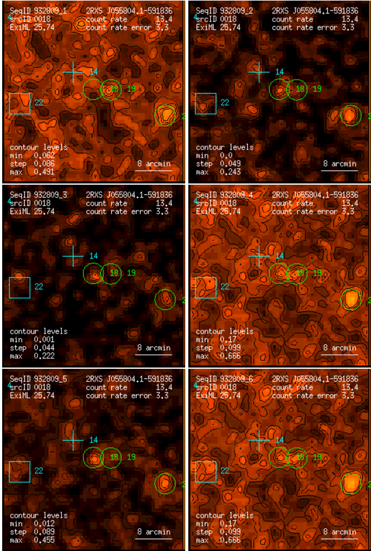
Figure 18: RASS 932809: detection 0018: band rate images, Gaussian filter: (1) PSPC channels 11 – 41, (2) 52 – 90, (3) 91 – 201, (4) 11 – 235, (5) 52 – 201, (6) 11 – 201. Broad band rates in counts/ks. Band rate contour levels in counts/ks/arcmin 2 .
