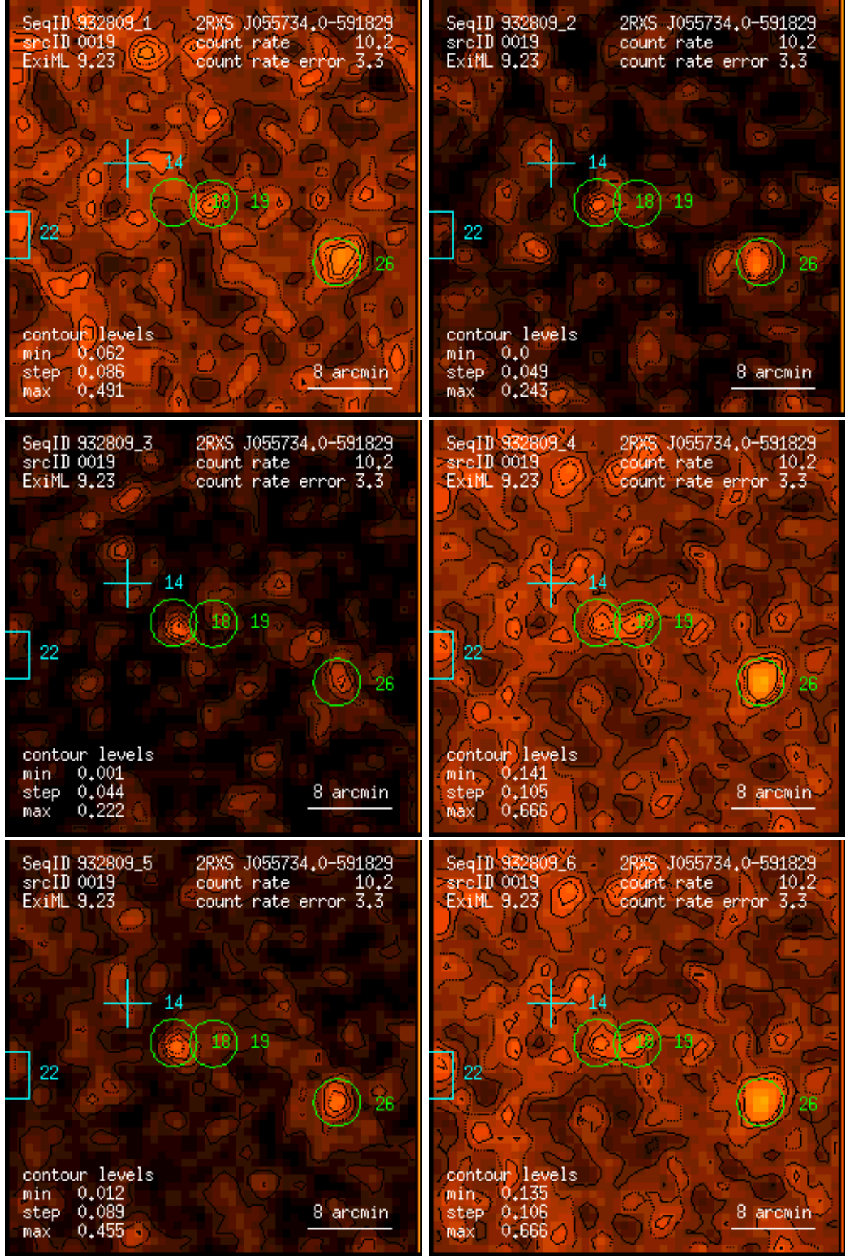
Figure 19: RASS 932809: detection 0019: band rate images, Gaussian filter: (1) PSPC channels 11 – 41, (2) 52 – 90, (3) 91 – 201, (4) 11 – 235, (5) 52 – 201, (6) 11 – 201. Broad band rates in counts/ks. Band rate contour levels in counts/ks/arcmin 2 .
