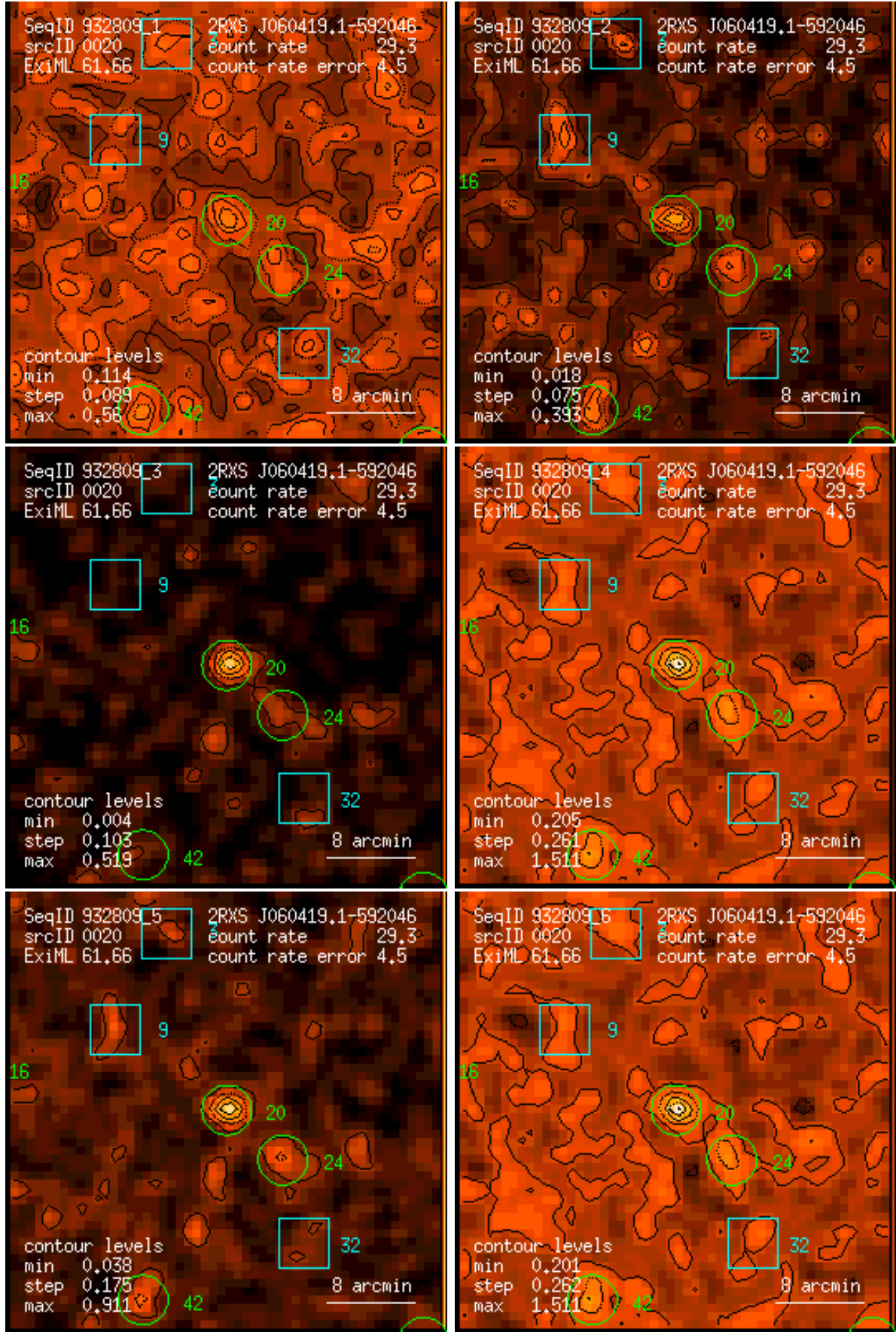
Figure 20: RASS 932809: detection 0020: band rate images, Gaussian filter: (1) PSPC channels 11 – 41, (2) 52 – 90, (3) 91 – 201, (4) 11 – 235, (5) 52 – 201, (6) 11 – 201. Broad band rates in counts/ks. Band rate contour levels in counts/ks/arcmin 2 .
