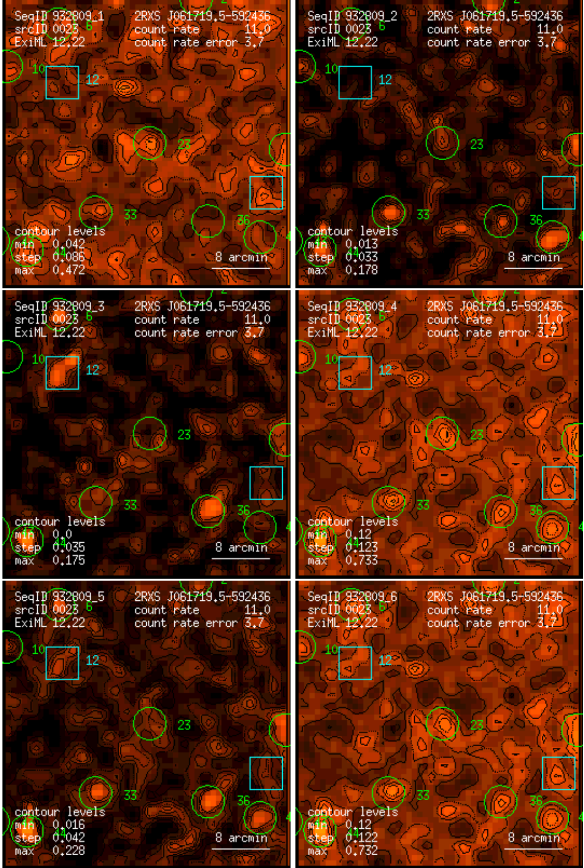
Figure 23: RASS 932809: detection 0023: band rate images, Gaussian filter: (1) PSPC channels 11 – 41, (2) 52 – 90, (3) 91 – 201, (4) 11 – 235, (5) 52 – 201, (6) 11 – 201. Broad band rates in counts/ks. Band rate contour levels in counts/ks/arcmin 2 .
