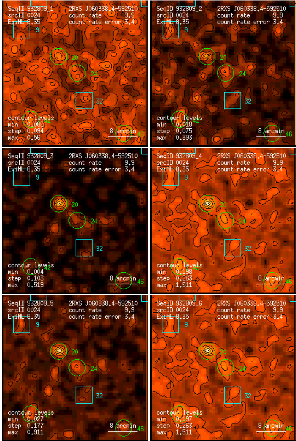
Figure 24: RASS 932809: detection 0024: band rate images, Gaussian filter: (1) PSPC channels 11 – 41, (2) 52 – 90, (3) 91 – 201, (4) 11 – 235, (5) 52 – 201, (6) 11 – 201. Broad band rates in counts/ks. Band rate contour levels in counts/ks/arcmin 2 .
