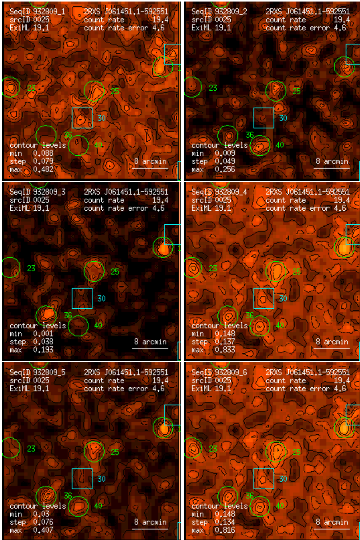
Figure 25: RASS 932809: detection 0025: band rate images, Gaussian filter: (1) PSPC channels 11 – 41, (2) 52 – 90, (3) 91 – 201, (4) 11 – 235, (5) 52 – 201, (6) 11 – 201. Broad band rates in counts/ks. Band rate contour levels in counts/ks/arcmin 2 .
