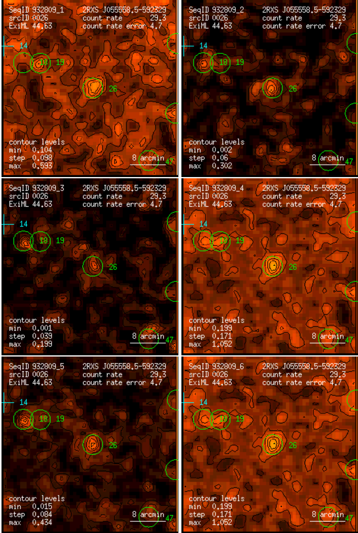
Figure 26: RASS 932809: detection 0026: band rate images, Gaussian filter: (1) PSPC channels 11 – 41, (2) 52 – 90, (3) 91 – 201, (4) 11 – 235, (5) 52 – 201, (6) 11 – 201. Broad band rates in counts/ks. Band rate contour levels in counts/ks/arcmin 2 .
