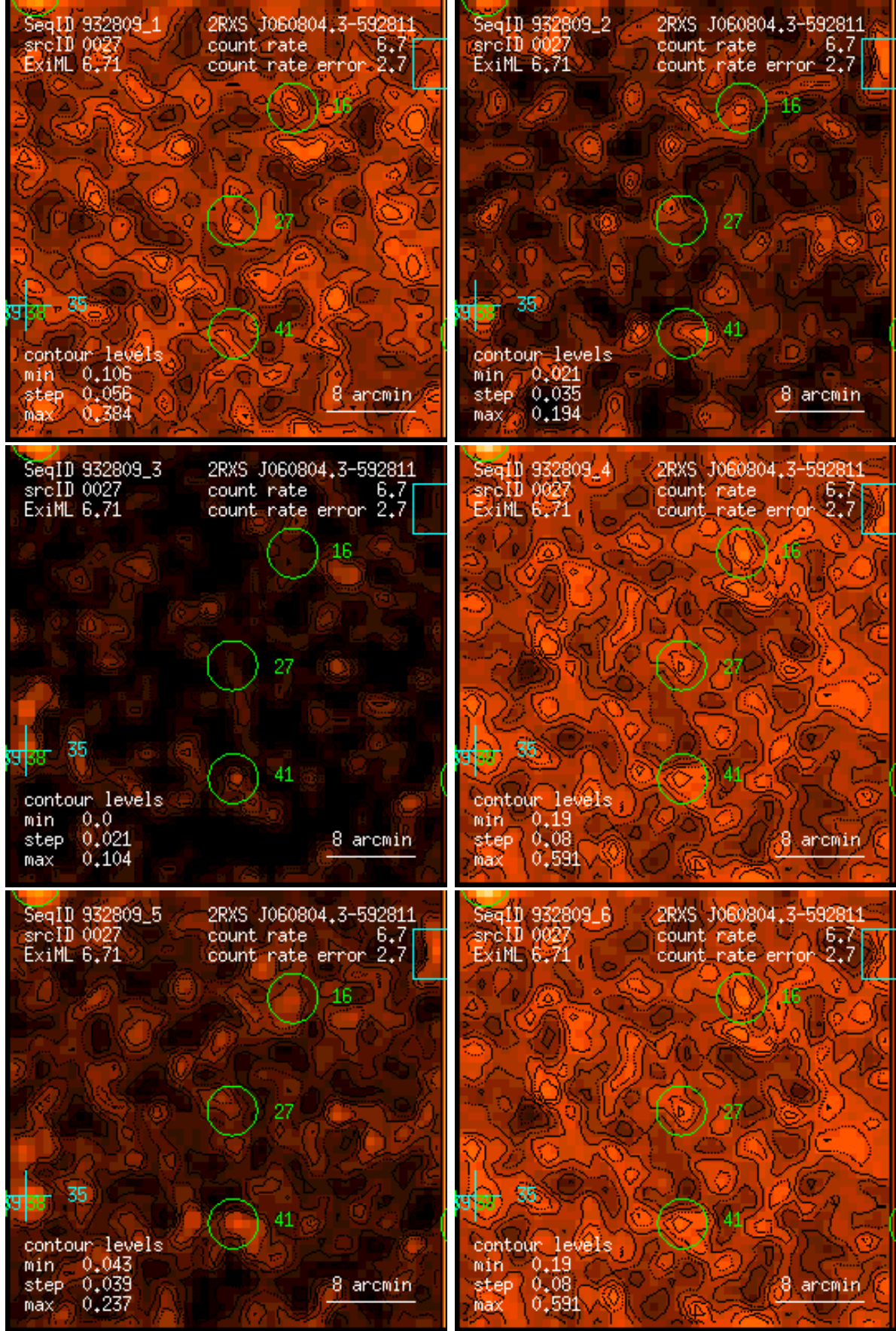
Figure 27: RASS 932809: detection 0027: band rate images, Gaussian filter: (1) PSPC channels 11 – 41, (2) 52 – 90, (3) 91 – 201, (4) 11 – 235, (5) 52 – 201, (6) 11 – 201. Broad band rates in counts/ks. Band rate contour levels in counts/ks/arcmin 2 .
