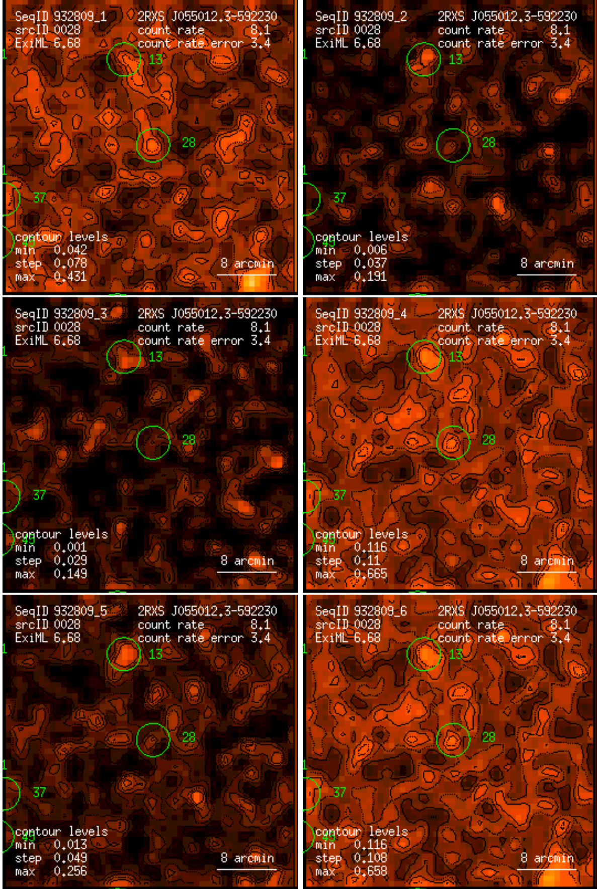
Figure 28: RASS 932809: detection 0028: band rate images, Gaussian filter: (1) PSPC channels 11 – 41, (2) 52 – 90, (3) 91 – 201, (4) 11 – 235, (5) 52 – 201, (6) 11 – 201. Broad band rates in counts/ks. Band rate contour levels in counts/ks/arcmin 2 .
