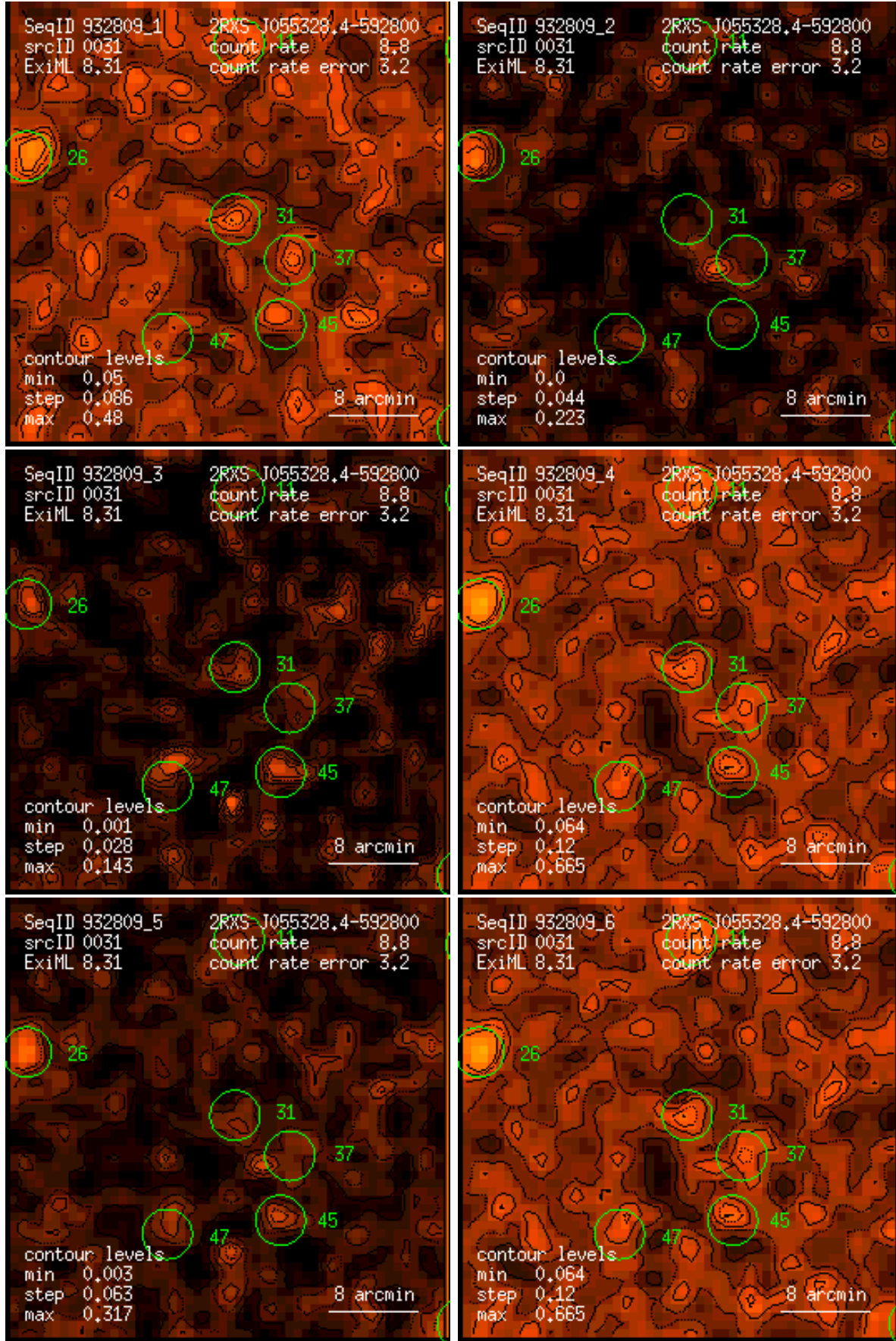
Figure 31: RASS 932809: detection 0031: band rate images, Gaussian filter: (1) PSPC channels 11 – 41, (2) 52 – 90, (3) 91 – 201, (4) 11 – 235, (5) 52 – 201, (6) 11 – 201. Broad band rates in counts/ks. Band rate contour levels in counts/ks/arcmin 2 .
