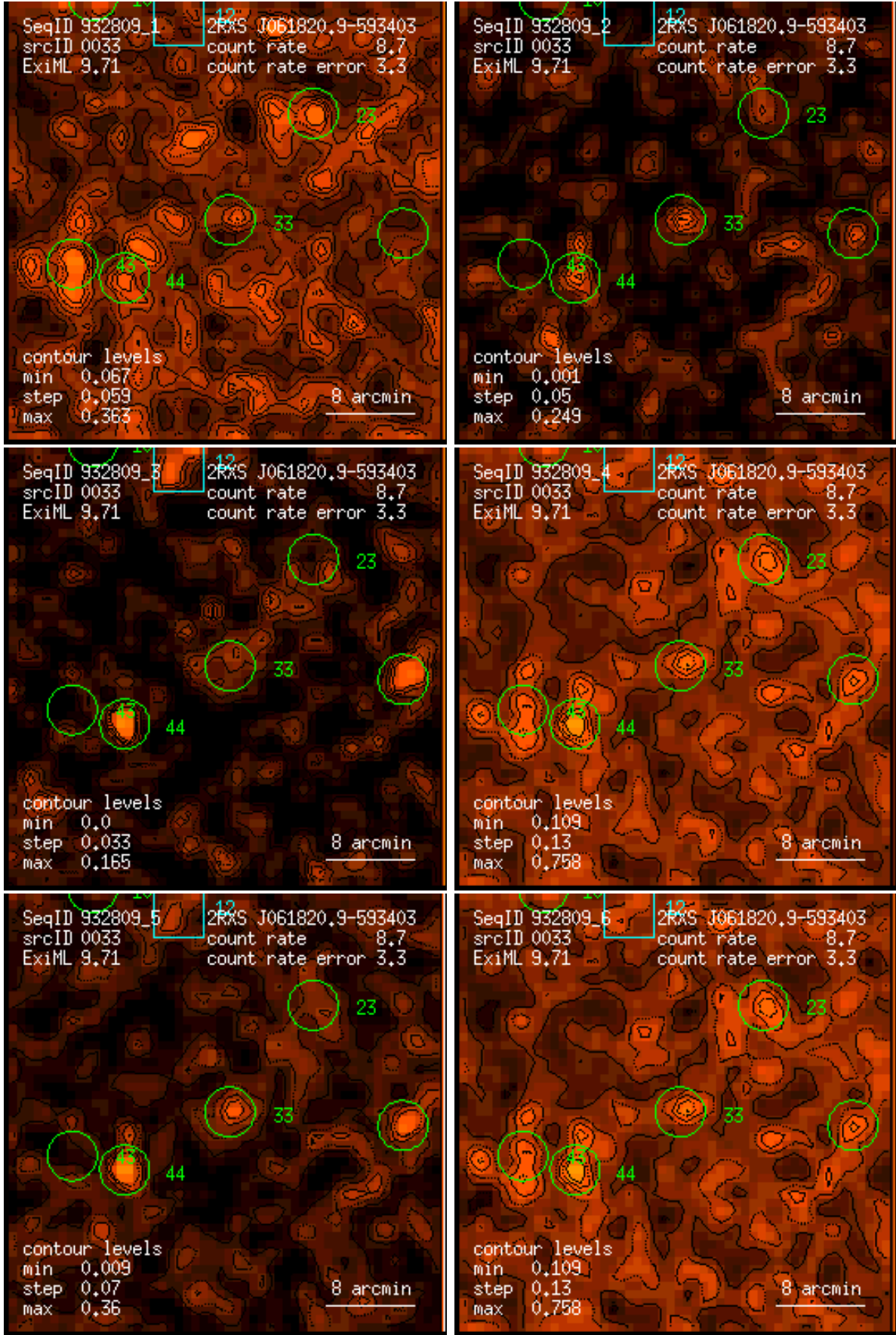
Figure 33: RASS 932809: detection 0033: band rate images, Gaussian filter: (1) PSPC channels 11 – 41, (2) 52 – 90, (3) 91 – 201, (4) 11 – 235, (5) 52 – 201, (6) 11 – 201. Broad band rates in counts/ks. Band rate contour levels in counts/ks/arcmin 2 .
