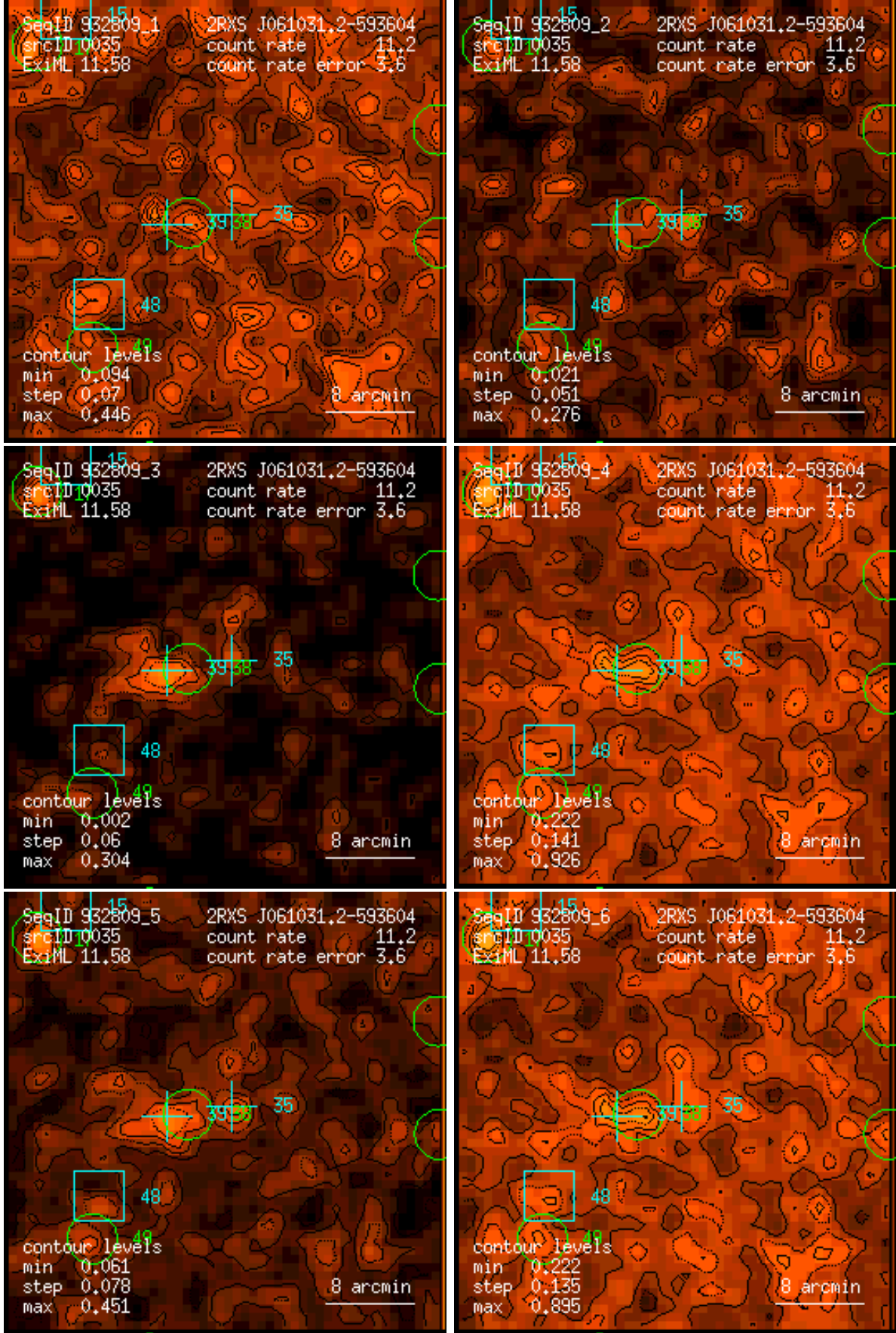
Figure 35: RASS 932809: detection 0035: band rate images, Gaussian filter: (1) PSPC channels 11 – 41, (2) 52 – 90, (3) 91 – 201, (4) 11 – 235, (5) 52 – 201, (6) 11 – 201. Broad band rates in counts/ks. Band rate contour levels in counts/ks/arcmin 2 .
